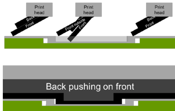
Figure 11 – Slitted Squeegee with front and back blade
