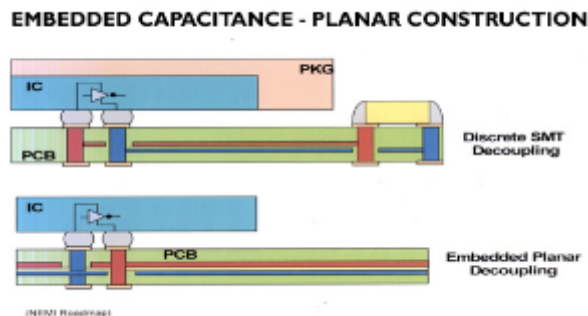
Figure 4 – Buried Capacitance Inside PCB 3
