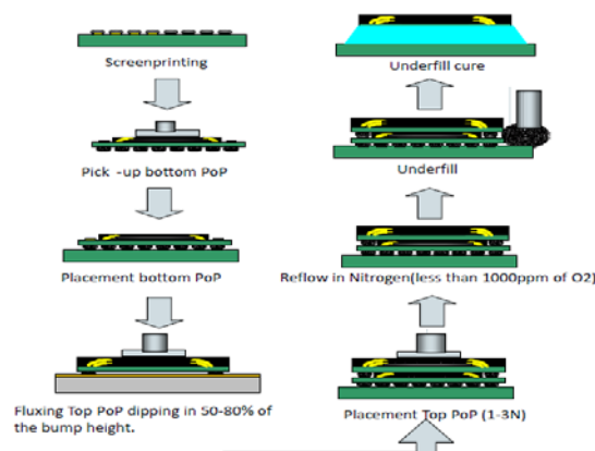
Figure 6 – PoP In-Line Process Flow
