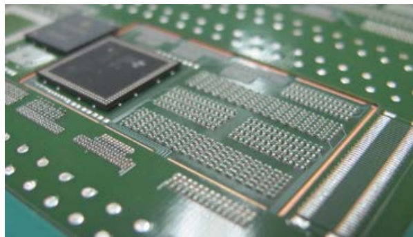
Figure 9 – Cavity Assembly
