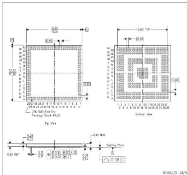
CBS (S-PBGA-N547)
