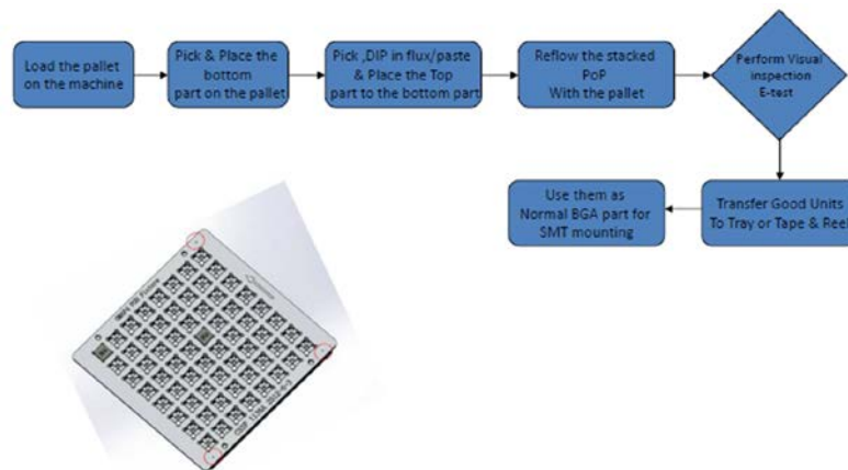
Figure 7 – PoP Pre-Stack General Process Flow
