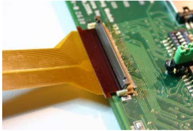
Figure 2 – Board to FPC using connector
