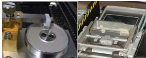
Figure 8 – Dipping Station: Rotary Drum (left), linear squeegee (right)
