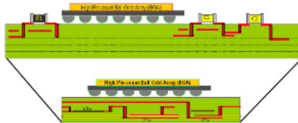
Figure 5 – Embedded Passives inside PCB 3
