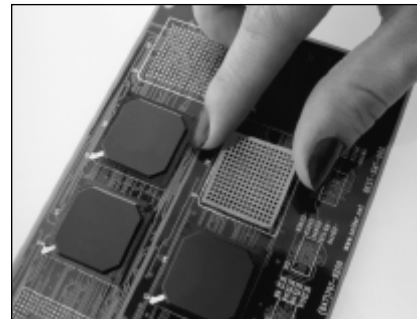
Figure 4. Semi-permanent stencil being placed onto a BGA site (BEST, Inc.).
