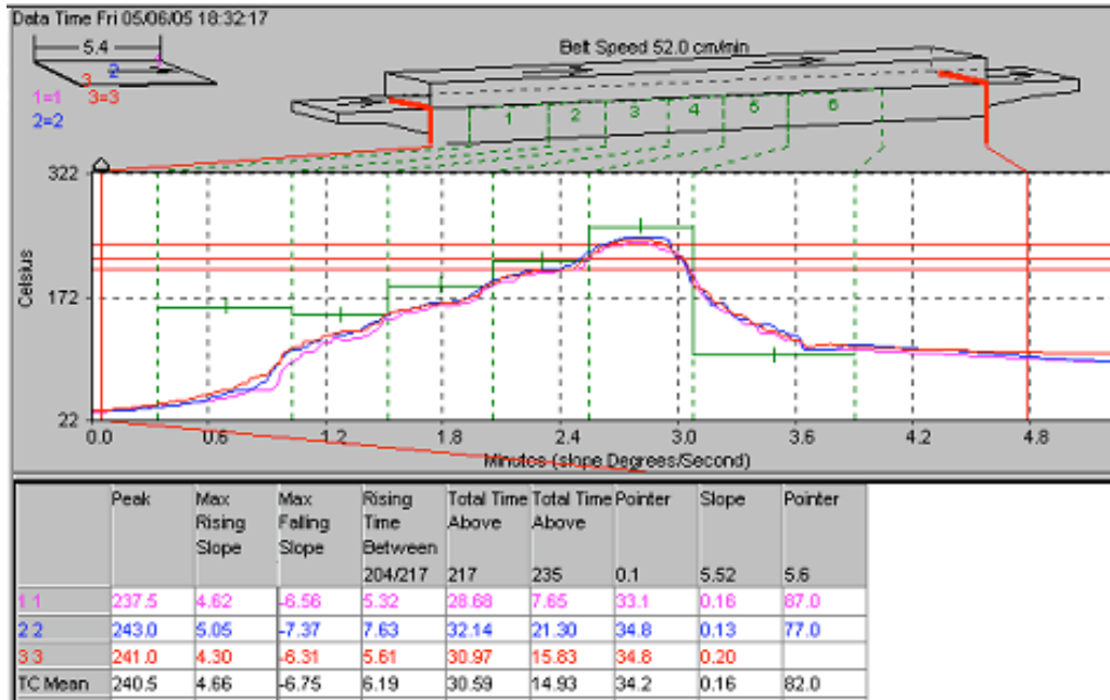
Figure 2. A sample lead-free reflow profile
