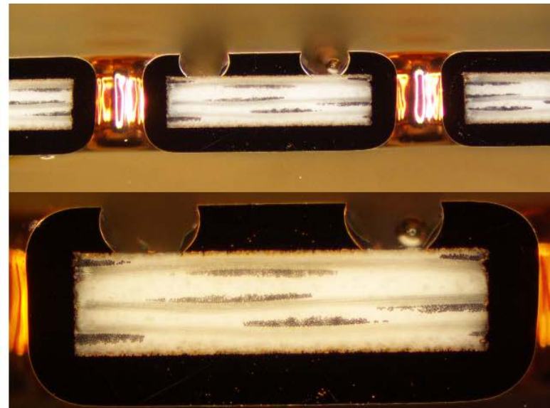
Tightly coupled GCPW with thick copper
