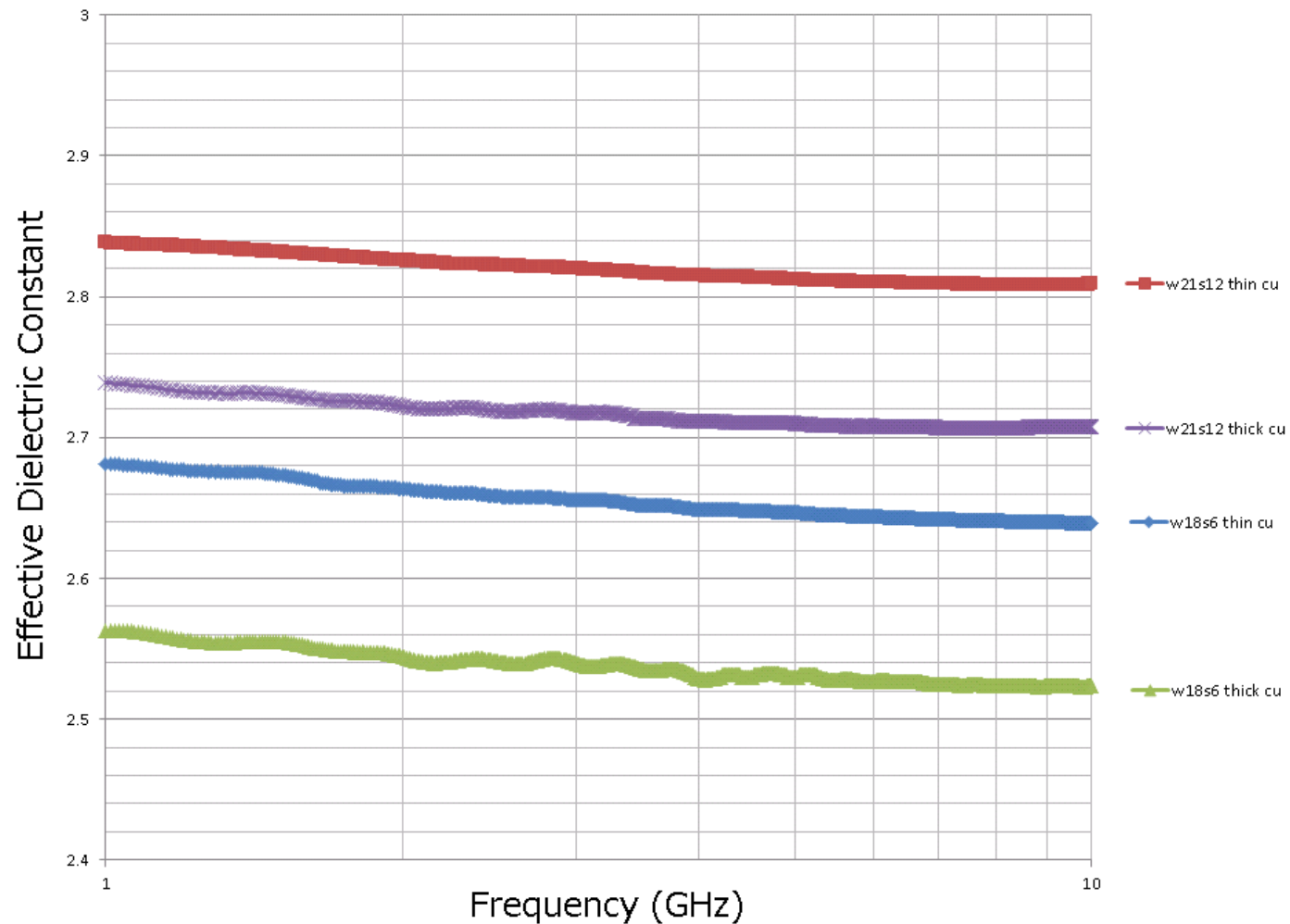
Grounded Coplanar Waveguide transmission line circuits using differential phase length method
