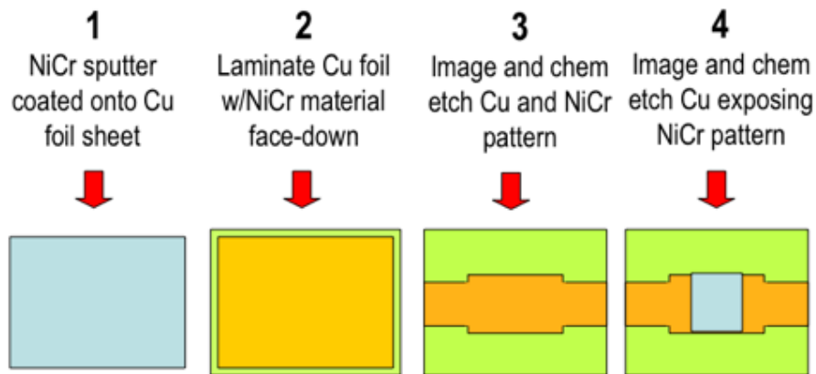
Figure 3- Thin-film resistor process sequence (Example source: IPC-7092)
