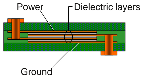
Sequential layer
