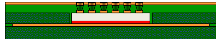
Laser ablate micro-vias
