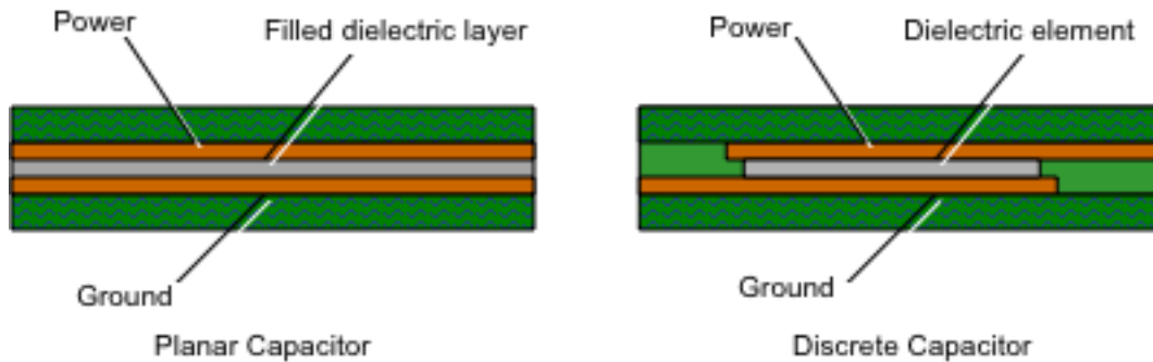
Figure 4- Planar and discrete capacitor elements (Example source: IPC-7092)
