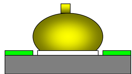
Gold ball bump
