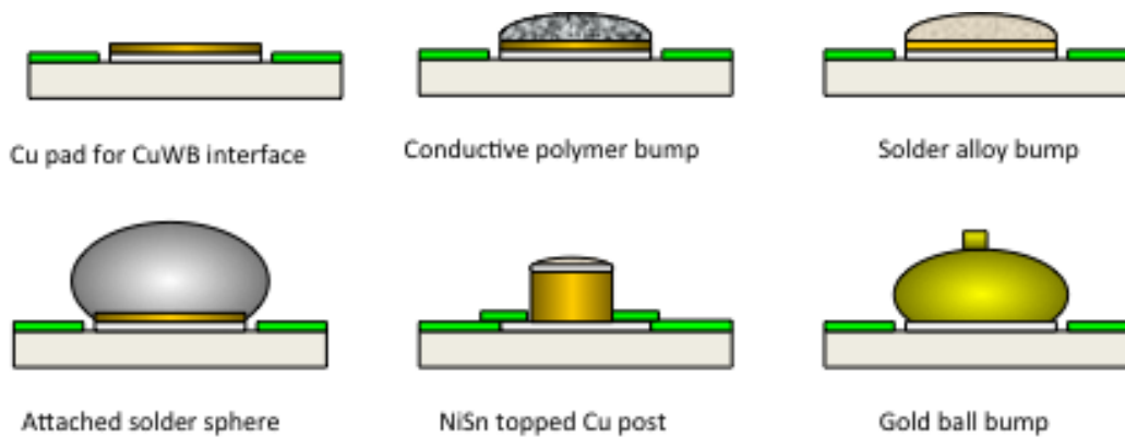
Figure 7- Semiconductor terminal variations for embedding
