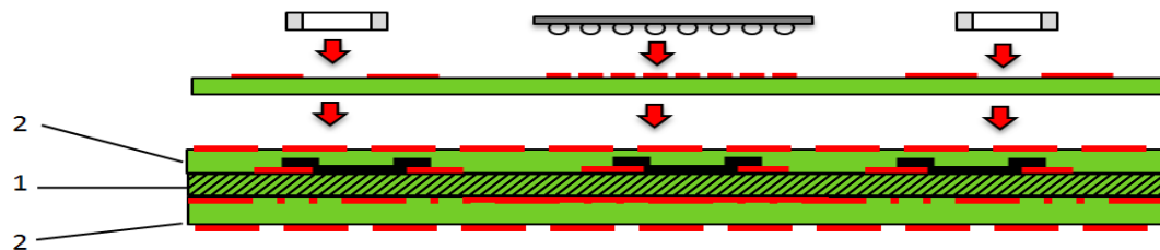
1-Copper clad (2 side) core; 2-Copper clad dielectric
