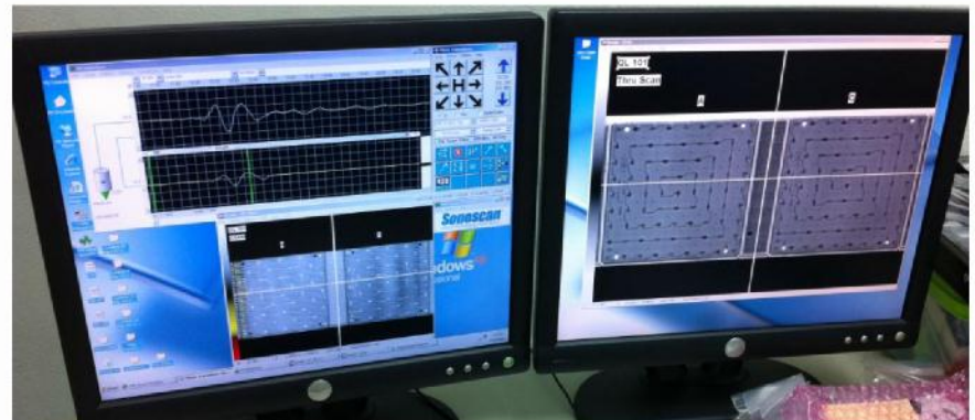
Fig7: Thru-scan in operation Fig8: Thru-scan imaging
