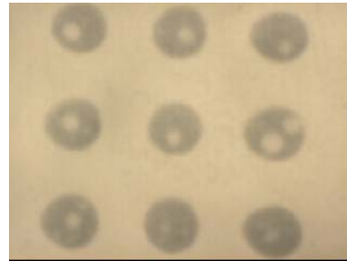
X-Ray, Voids in BGA 's
