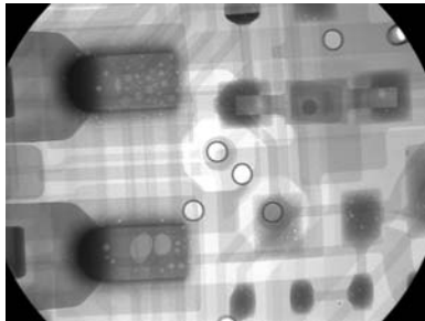
X-Ray, Voids in QFP joints
