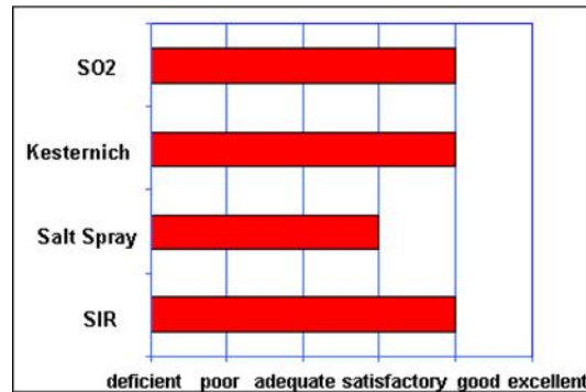
Fig. 17 Corrosion test results for ENIG (High P)
