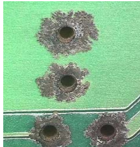
← Creep corrosion on ImAg protected vias*
