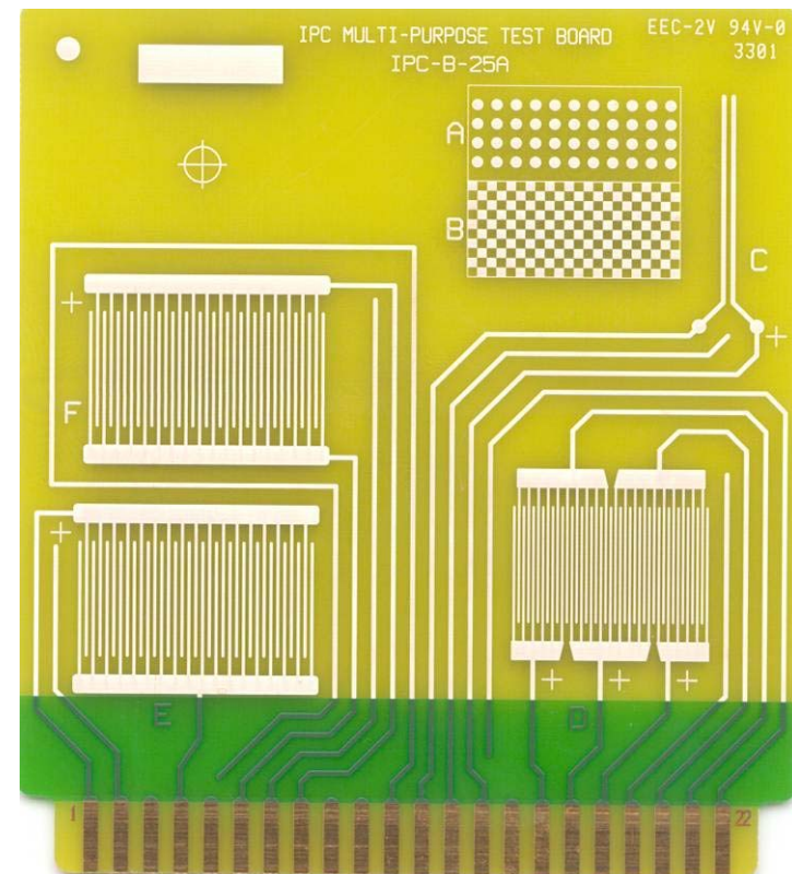
Surface Insulation - Test board
