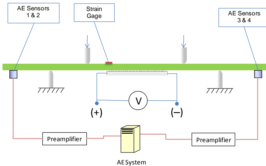
Figure 6 - Schematic of Bend Test Set-up with AE Sensors
