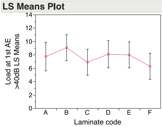
Figure 6. (a) The applied load at first locatable AE event with amplitude greater than 40 dB, (b) Average applied load when first four AE events with amplitude greater than 40 dB.
