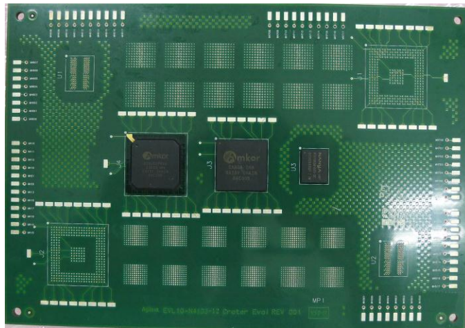
Figure 1: Test Coupon.
