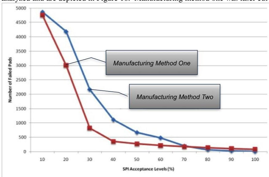
Figure 16 - Amount of solder paste misprints when comparing two different stencil manufacturing methods.
