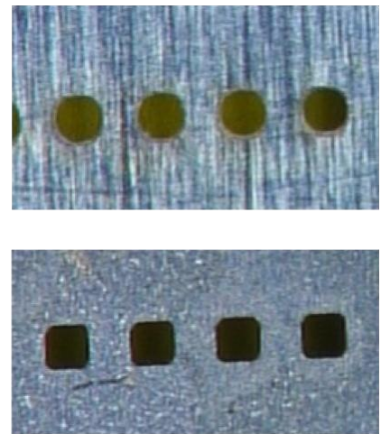
Figure 16 - Amount of solder paste misprints when comparing two different stencil manufacturing methods.
