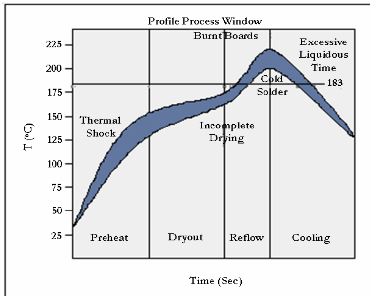
A Graphical representation of a 25°C reflow profile process band
