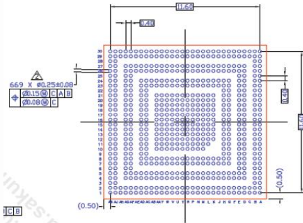
CSP component
