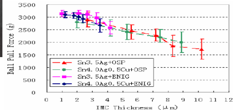
Figure 20. Effect of IMC thickness on the ball pull strength (Pull speed: 5000 µm/s)
