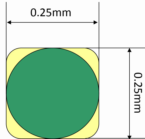
Stencil opening
