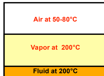
Vapor Phase temperatures for leaded soldering
