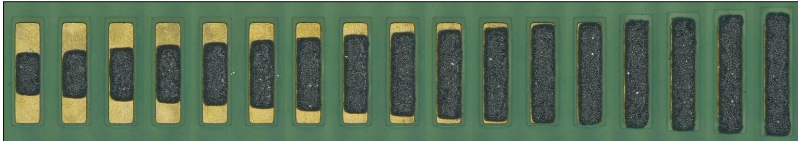
Solder Spread Test Coupon before Reflow (40% to 120% Solder Paste Coverage)
