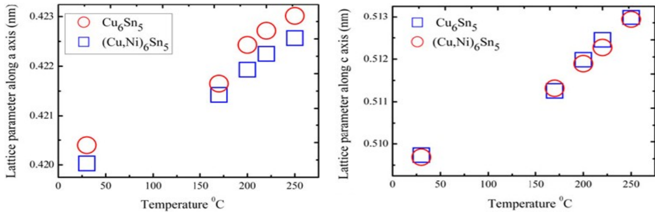
Figure 4. a and c axis lattice parameters in hexagonal \text{Cu}_6\text{Sn}_5 and (\text{Cu,Ni})_6\text{Sn}_5 as a function of temperature.[4]
