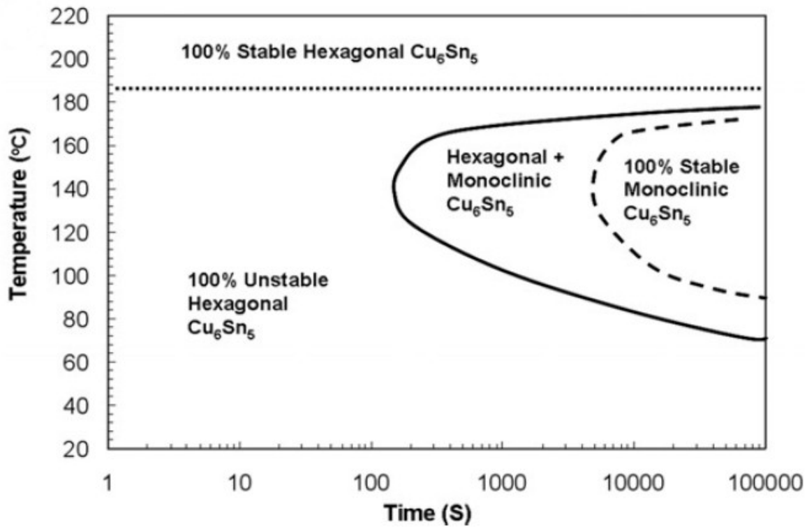
Figure 10. Estimated boundaries of Temperature-Time-Transformation (TTT) curves for \text{Cu}_6\text{Sn}_5 . [5]
