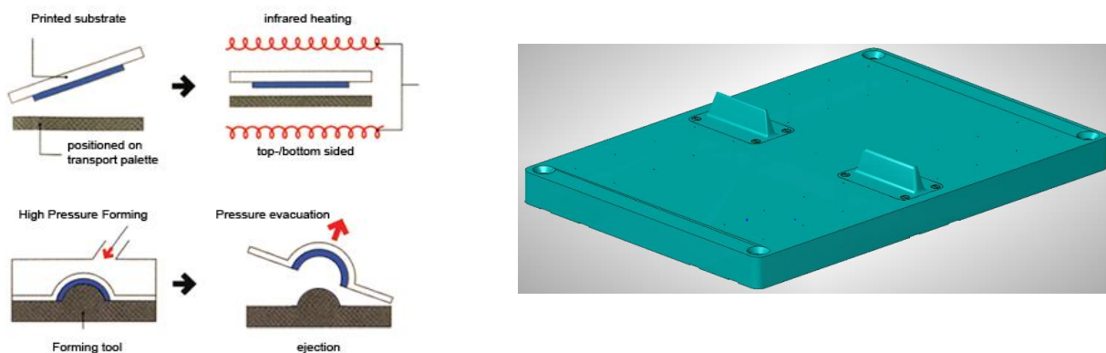
Figure 1 Schematic of a thermoforming process (left) and tooling plate (right)
