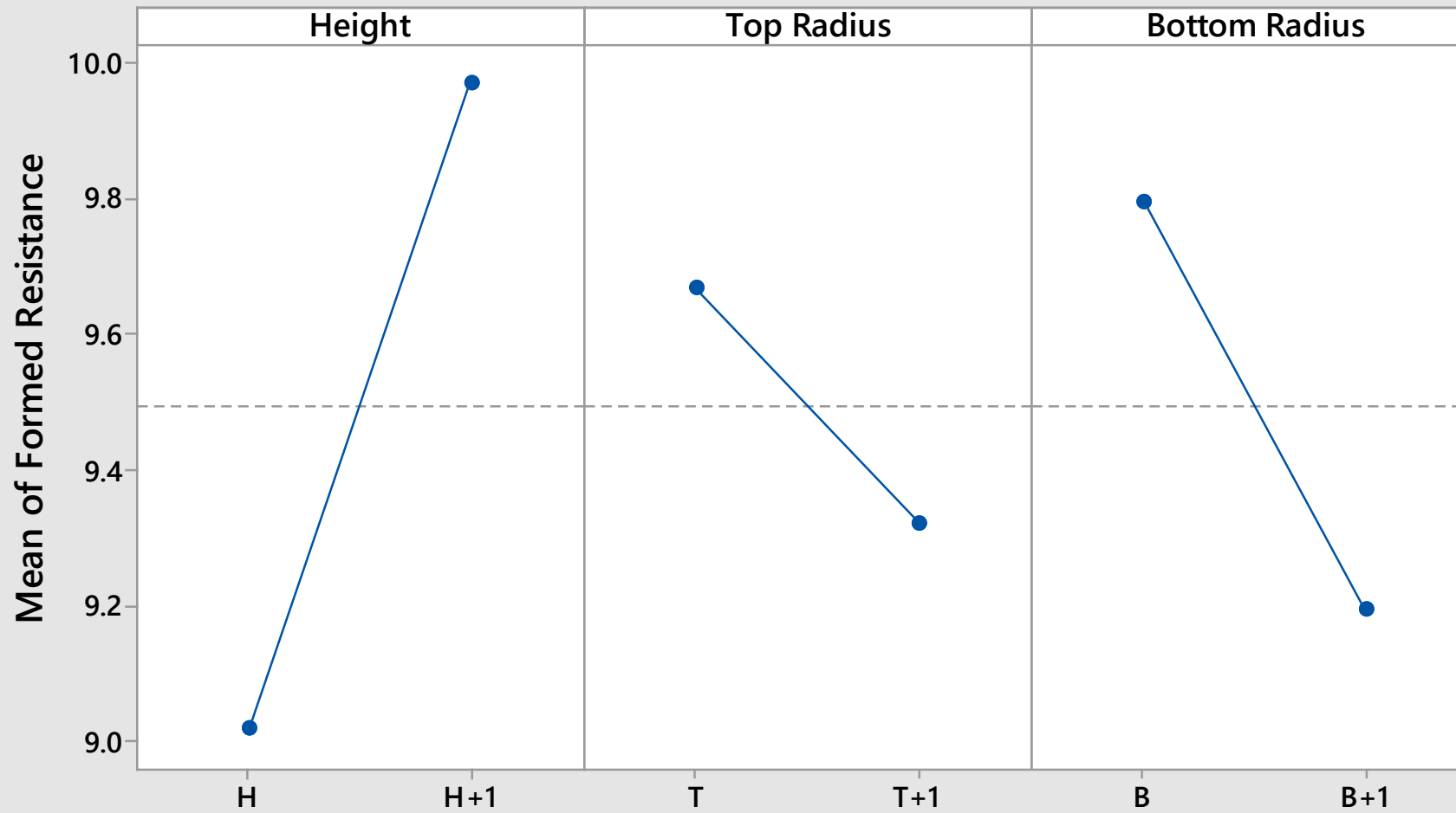
Factorial Plot Formed Resistance for X+4 Trace Fitted Means
