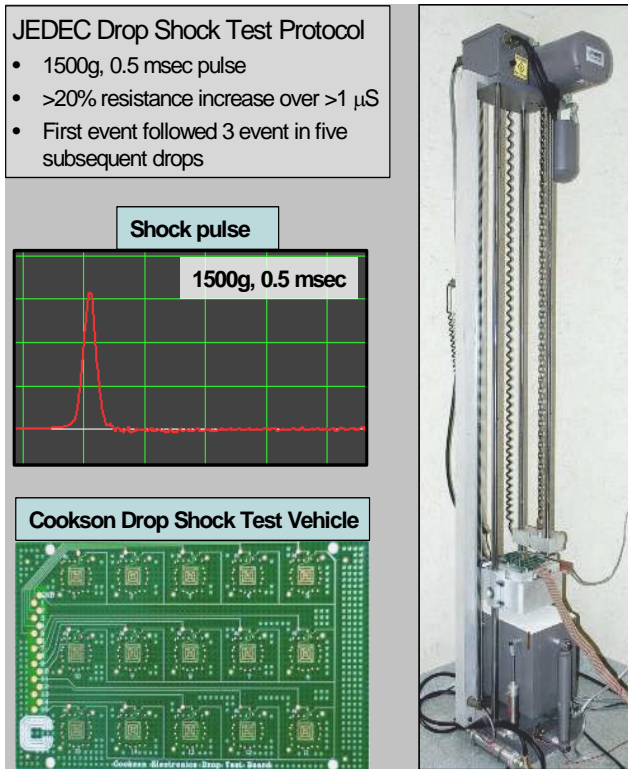
FIGURE 4: Drop shock system and JEDEC test protocol
