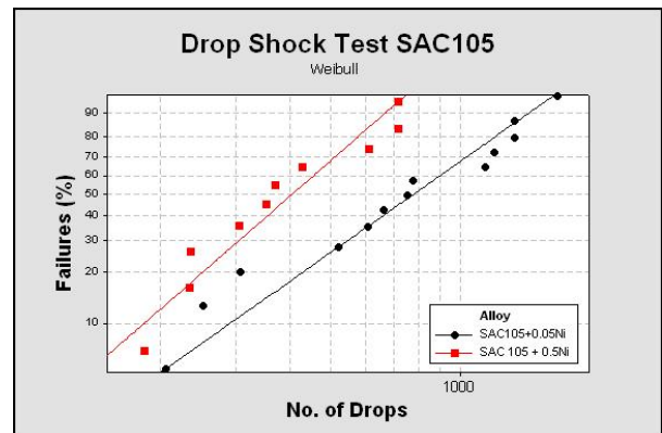
FIGURE 14: Drop shock data for SAC105 with 0.05% Ni and 0.5% Ni
