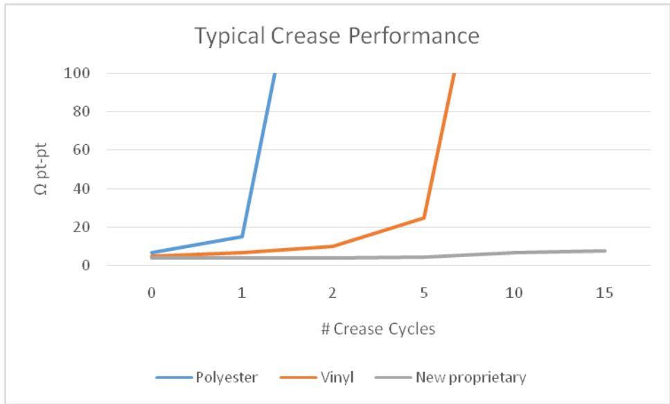
Figure 3. Crease test performance comparisons
