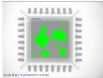
SAC301 18.5 T4 QFN I-O EXP-II RTS-L-H PCB#9 QFN32-2 IO_10MIL 29.12%
