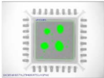
SAC305 8.5 T4 QFN I-O EXP-II RTS-L-H PCB#9 QFN32-1 STD_IO 13.49%
