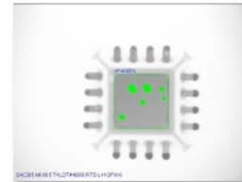
SAC30! 18.5 T4 QFN I-O EXP-II RTS-L-H PCB#9 QFN16-4 IO_30MIL 6.56%
