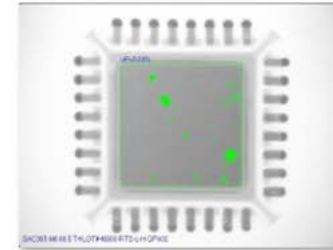
SAC301 18.5 T4 QFN I-O EXP-II RTS-L-H PCB#8 QFN32-4 IO_30MIL 2.24%
