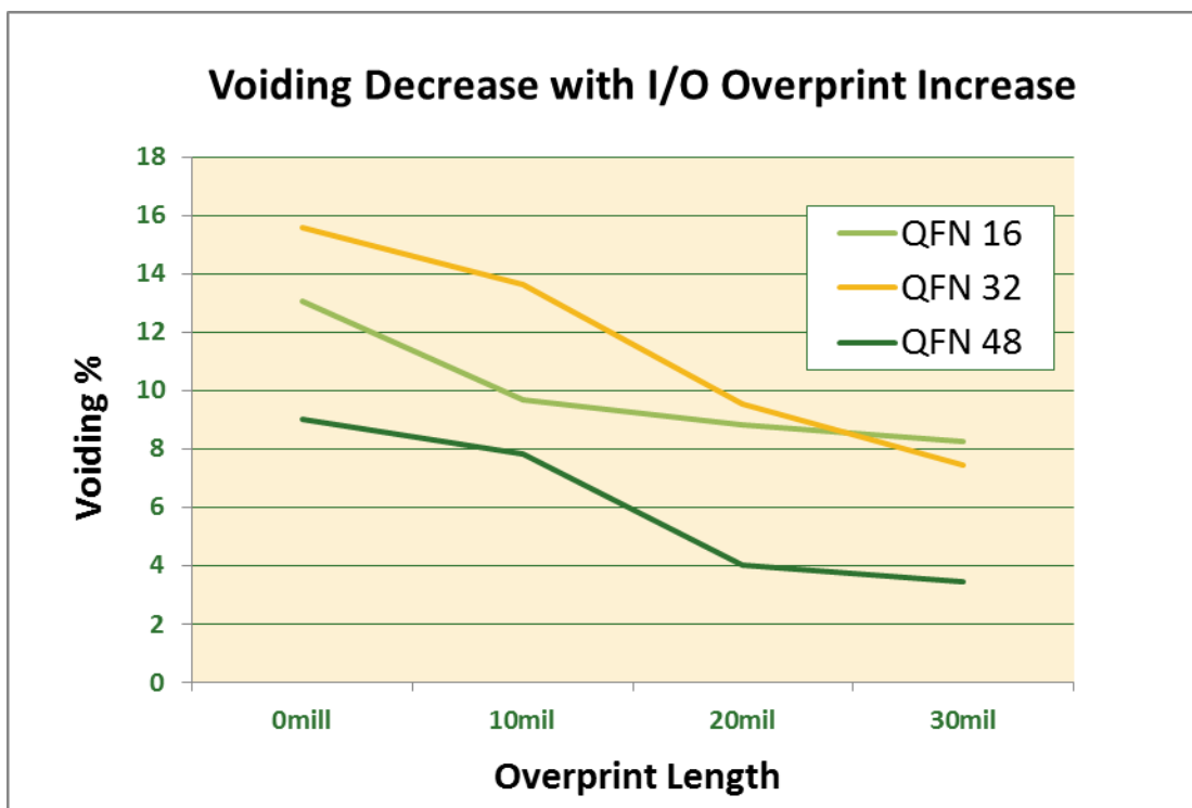
Figure 11 – Voiding Summary
