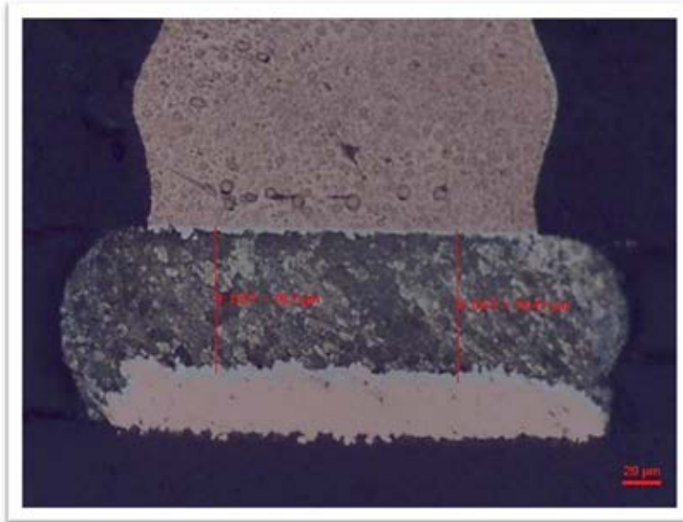
No Overprint 78.05μm
