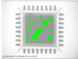
SAC301 18.5 T4 QFN I-O EXP-II RTS-L-H PCB#7 QFN32-2 IO_10MIL 18.61%
