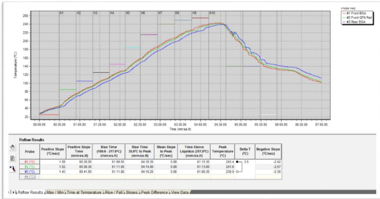
Figure 7 – Selected Profile
