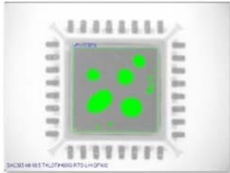
SAC305 1.5 T4 QFN I-O EXP-II RTS-L-H PCB#8 QFN32-1 STD_IO 17.32%
