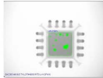
SAC305 8.5 T4 QFN I-O EXP-II RTS-L-H PCB#7 QFN16-3 IO_20MIL 7.58%
