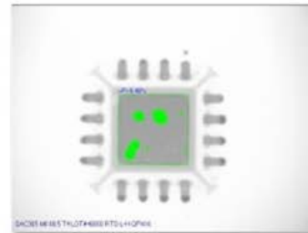
SAC30 18.5 T4 QFN I-O EXP-II RTS-L-H PCB#9 QFN16-3 IO_20MIL 9.48%
