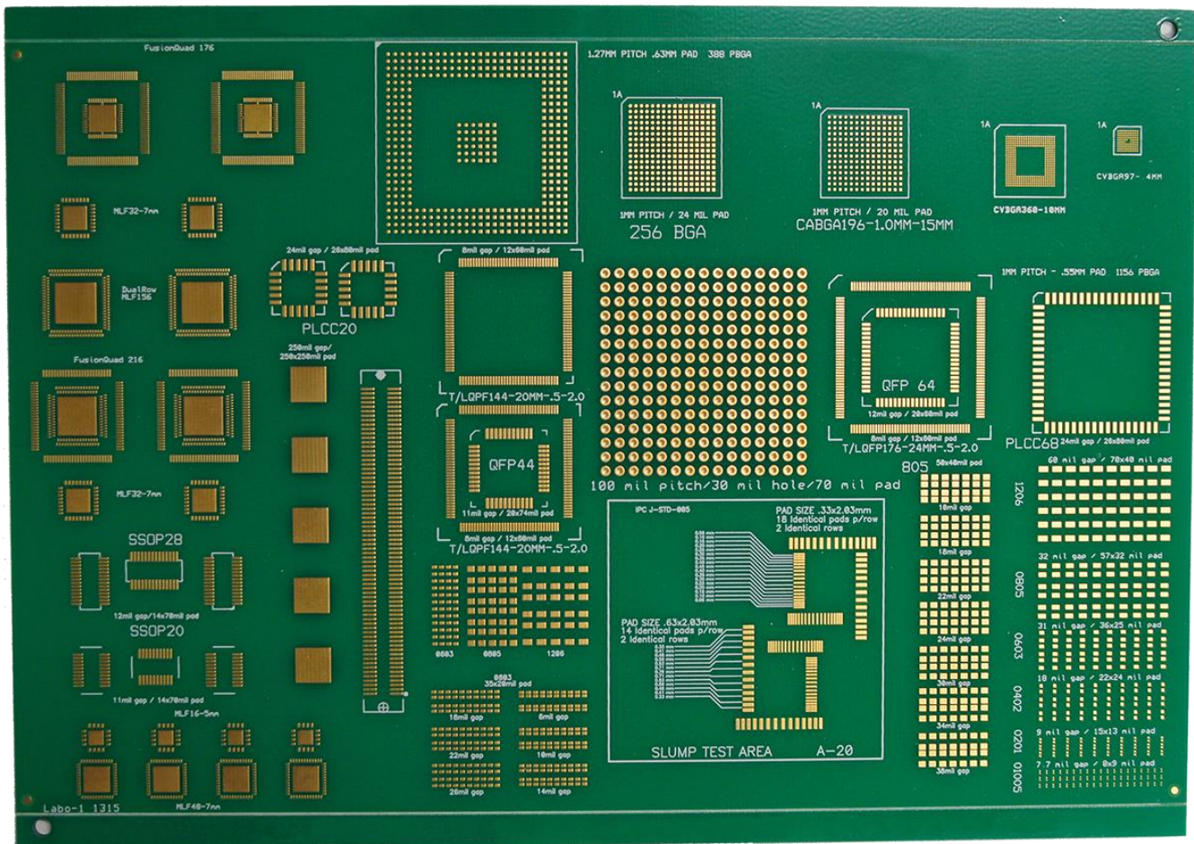
Figure 3 – Test Vehicle
