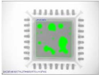
SAC305 8.5 T4 QFN I-O EXP-II RTS-L-H PCB#7 QFN32-1 STD_IO 21.80%
