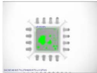
SAC305 8.5 T4 QFN I-O EXP-II RTS-L-H PCB#9 QFN16-2 IO_10MIL 18.44%
