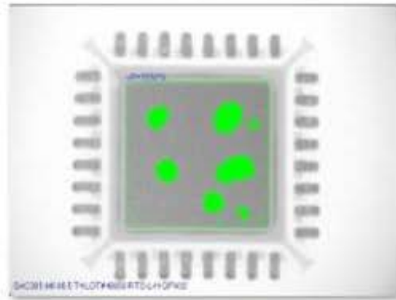
SAC305 88.5 T4 QFN I-O EXP-II RTS-L-H PCB#8 QFN32-2 IO_10MIL 13.52%
