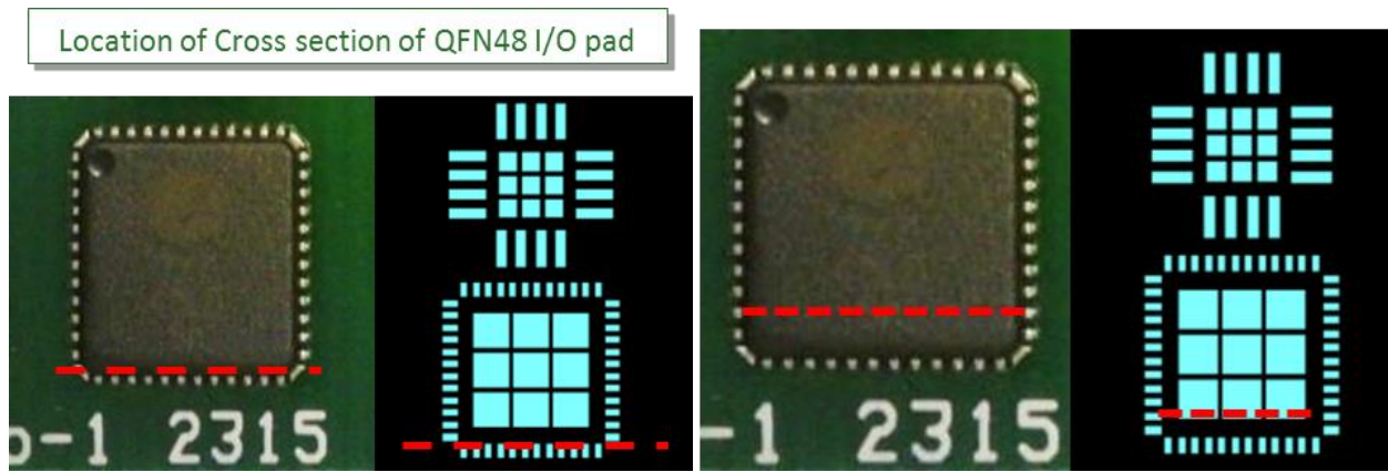
Figure 12 – Locations of Cross-sections on MLF48
