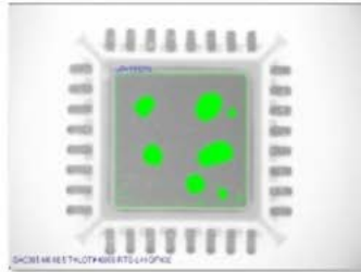
SAC301 18.5 T4 QFN I-O EXP-II RTS-L-H PCB#8 QFN32-2 IO_10MIL 13.52%
