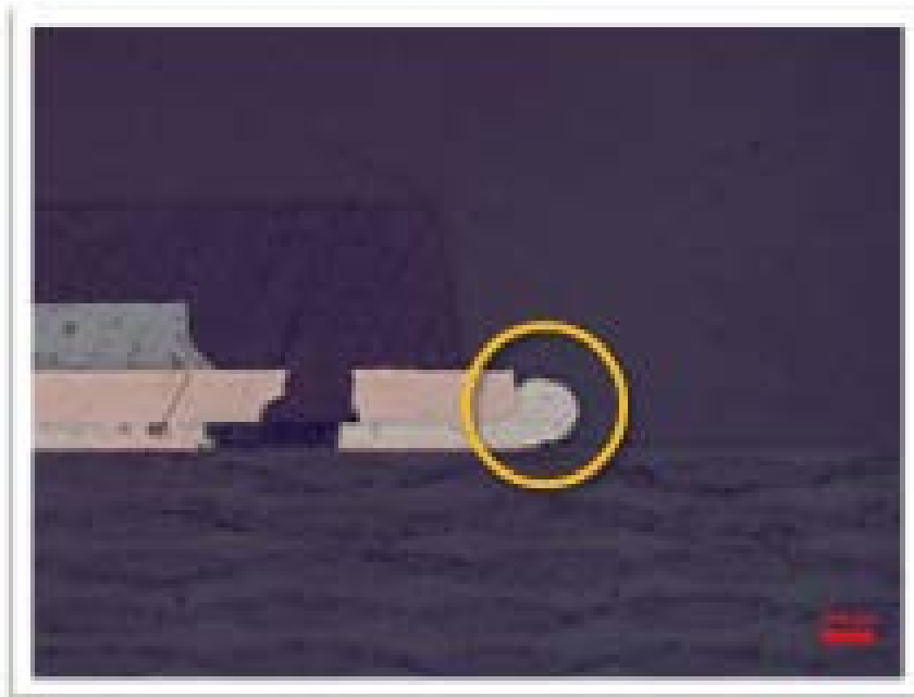
30mil Overprint Potential Excessive
