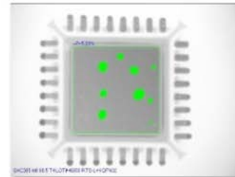
SAC305 3.5 T4 QFN I-O EXP-II RTS-L-H PCB#9 QFN32-3 IO_20MIL 5.23%
