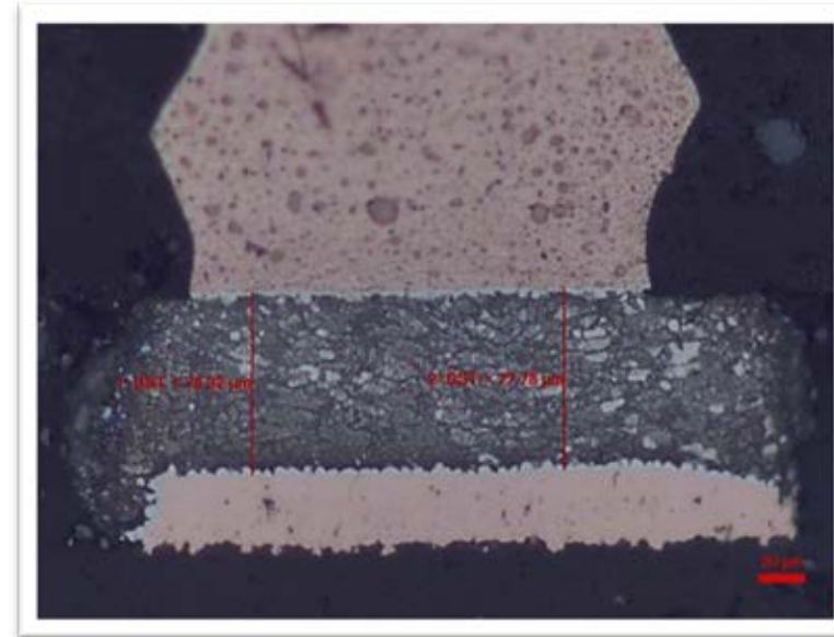
30mil Overprint 78.06μm
