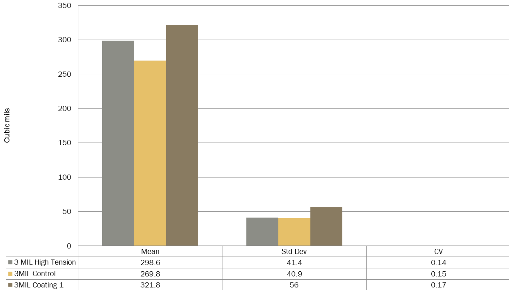
Solder Paste Volume 0201 Component-3 mil stencil
