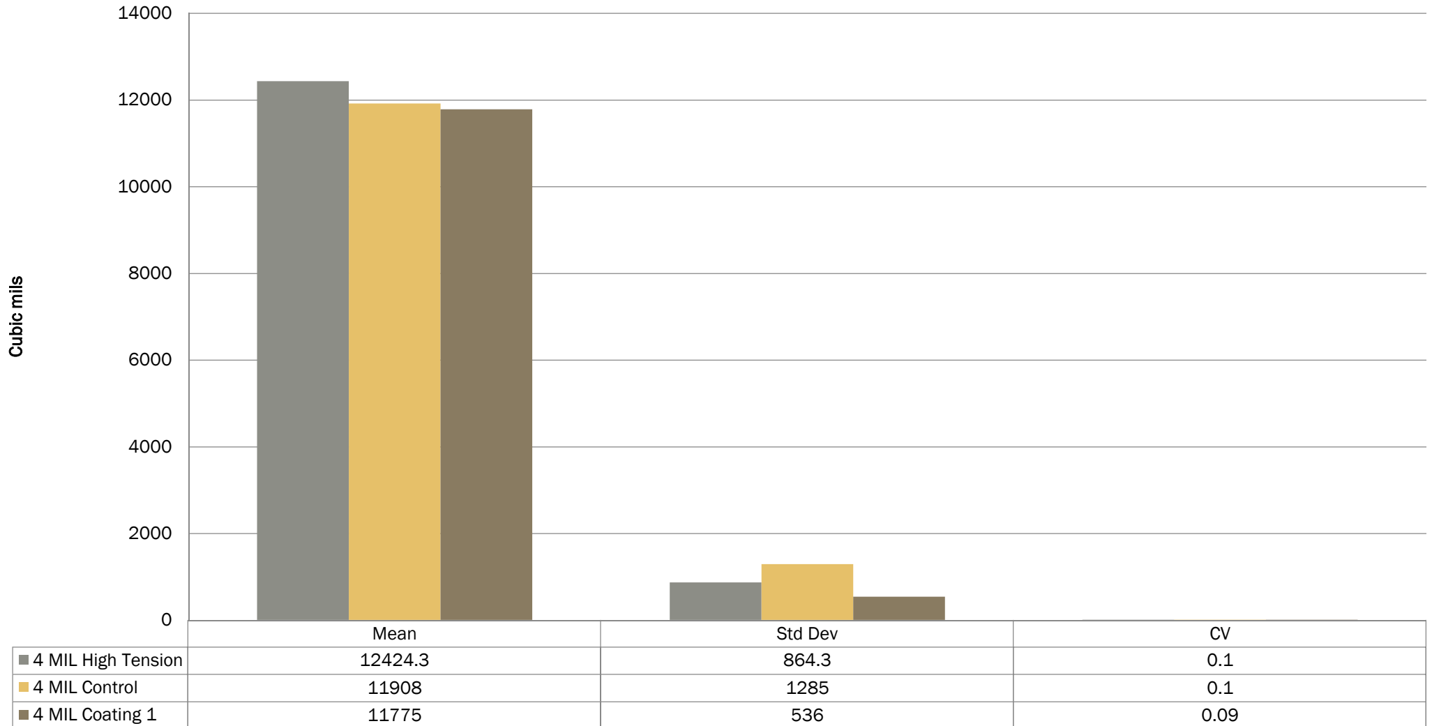
Solder Paste Volume 1206 Component-4 mil stencil
