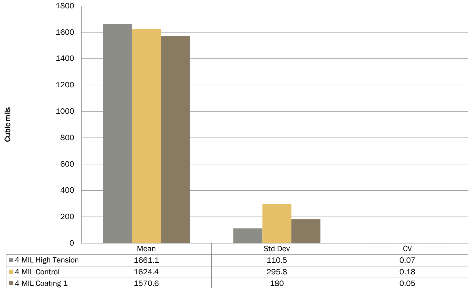
Solder Paste Volume 0402 Component-4 mil stencil
