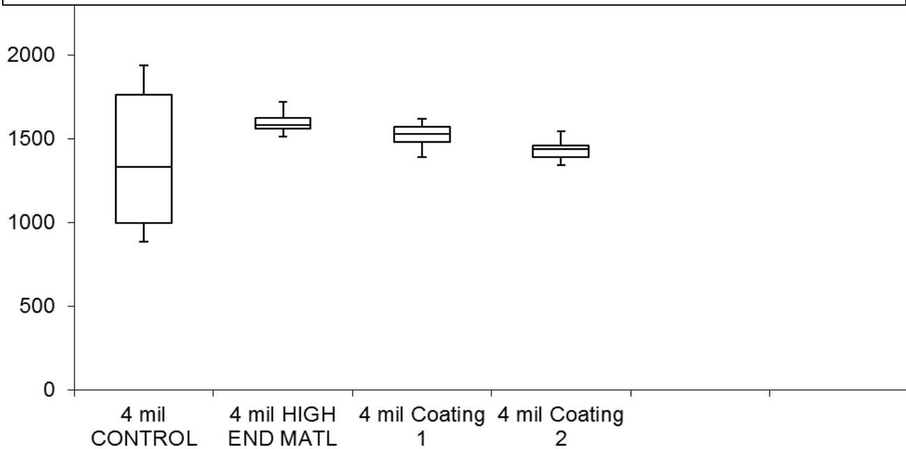
Figure 9- Box plot of print performance , 4 mil stencils, 0402-22 x 24 mil pad size
