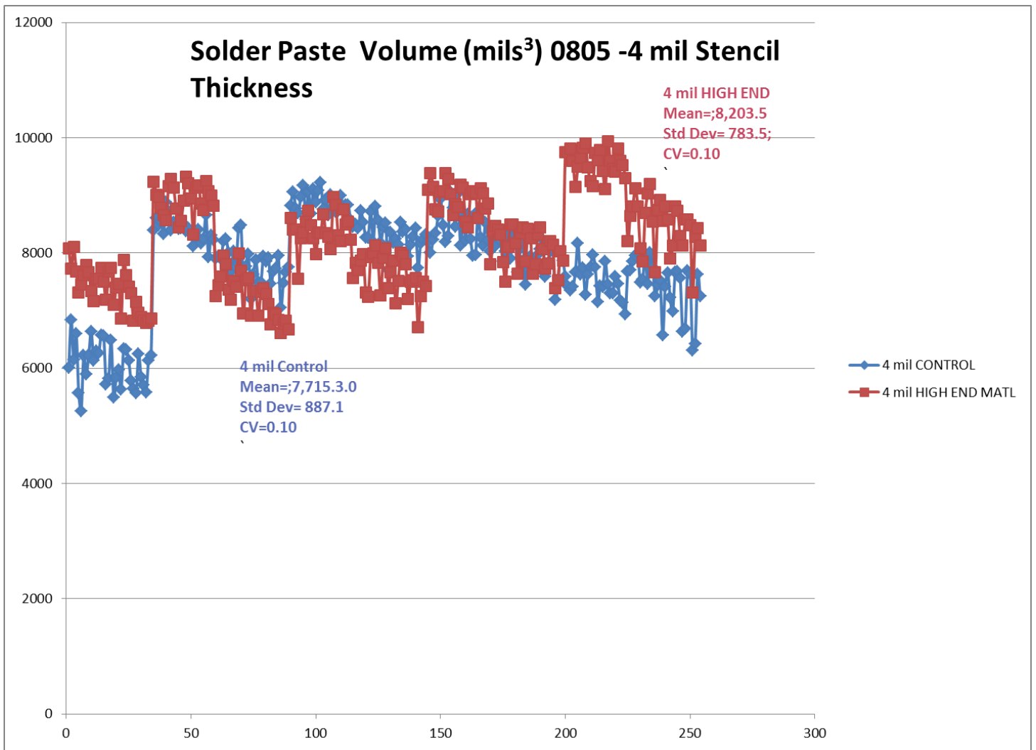
Figure 6- Print performance , 4 mil stencils, Various stencils 0805-46.6 X 37.0 mil measured aperture size
