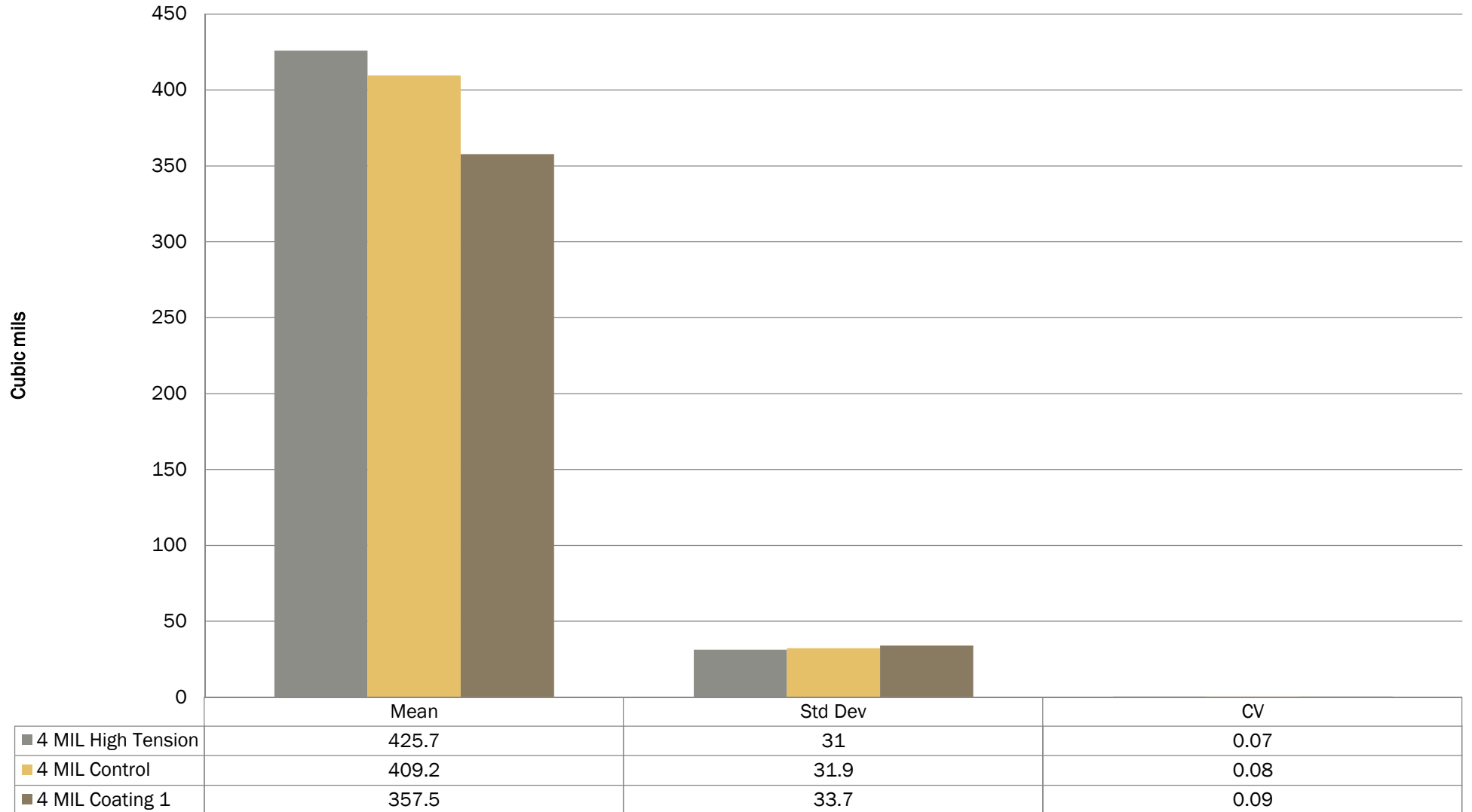
Solder Paste Volume 0201 Component-4 mil stencil
