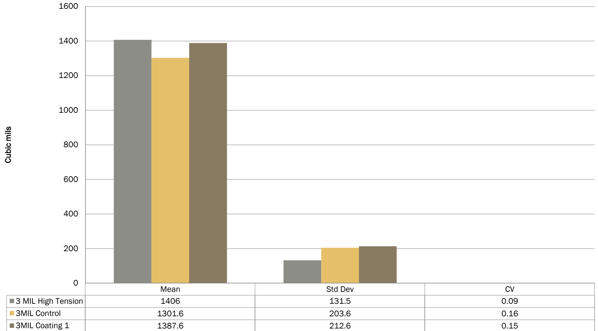
Solder Paste Volume 0402 Component-3 mil stencil
