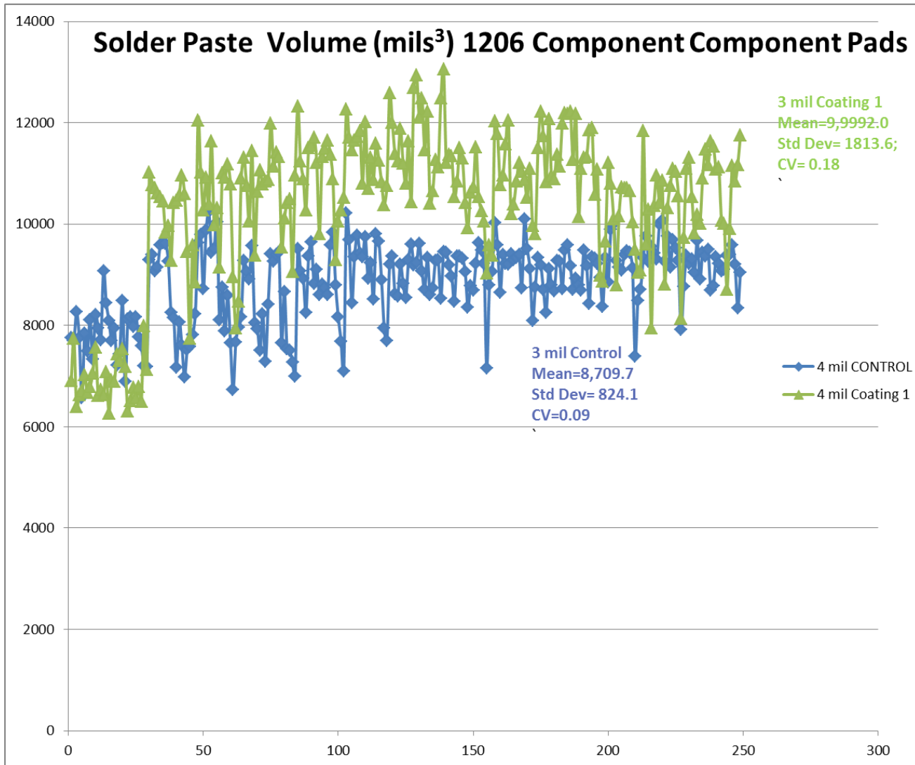
Figure 7- Print performance, 4 mil stencils, Various stencils 1206- 62.8 X 37.0 mil pad size
