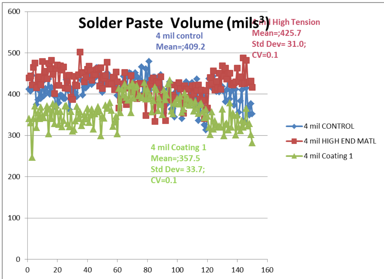
Figure 8- Print performance, 4 mil stencils, Various stencils 0201-12.0x10.1 mil pad size
