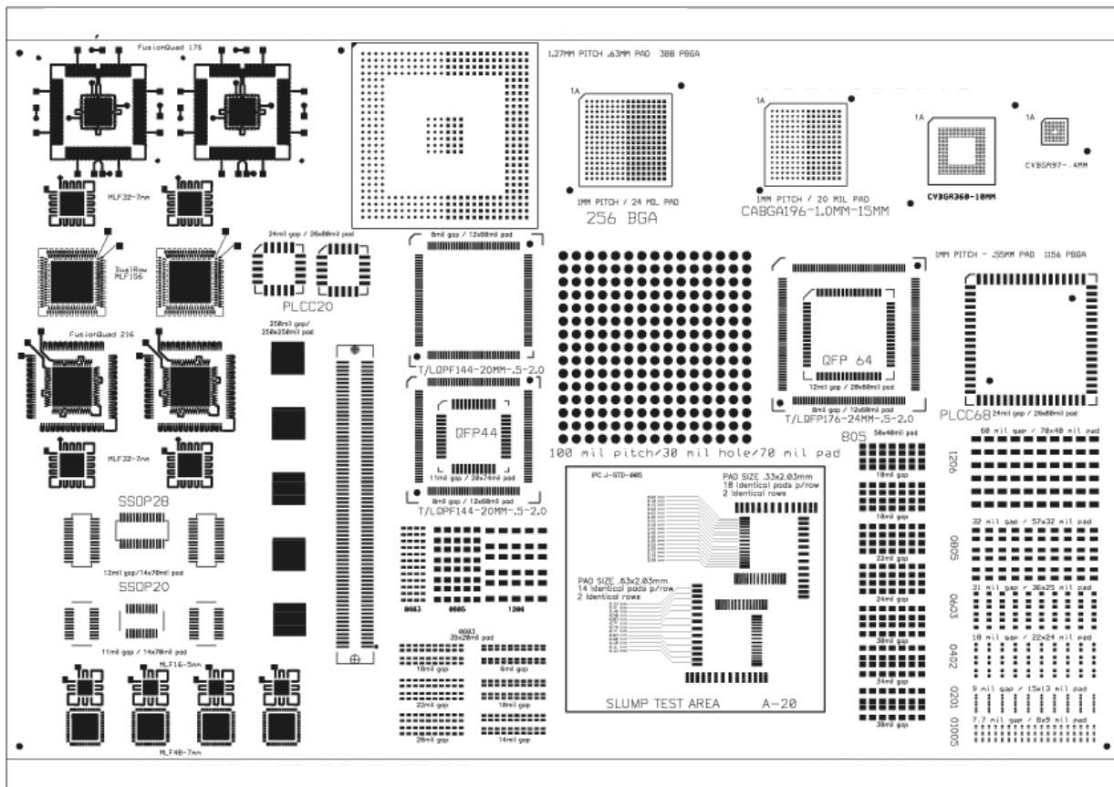
Figure 1: Solder paste Evaluation Board Layout
