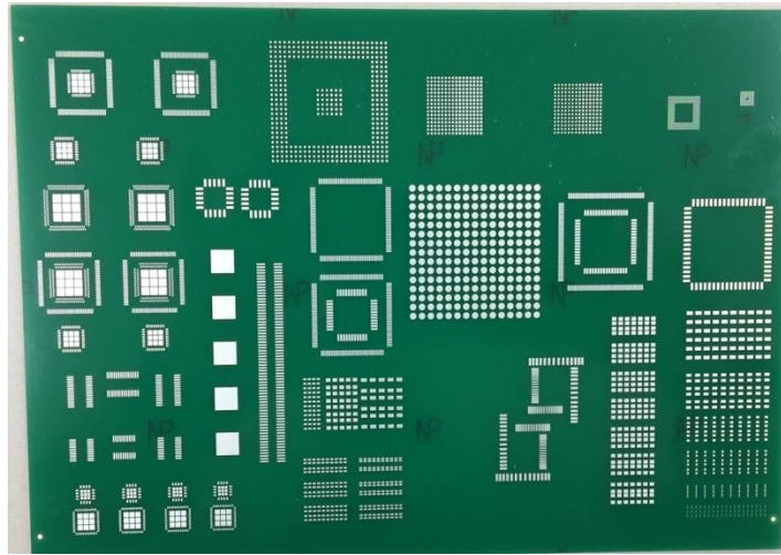
Figure 2: Test Vehicle for Solder Paste Printing Study
