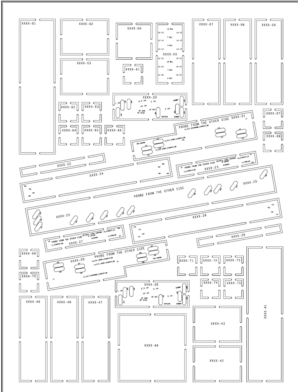
Figure 2: Final Test Board Layout
