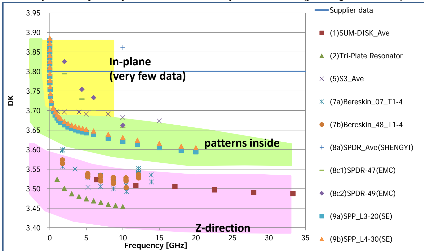
Comparison of Dk/Df Extraction Results by Test Method (for single material)
