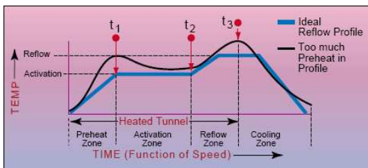
Fig.6. Too much preheat, decrease temp in preheat zone.
