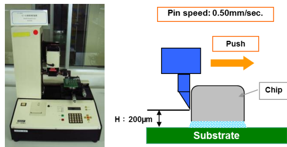
Figure 4 - Bond Tester Equipment (Left) and Schematic of test method(Right)
