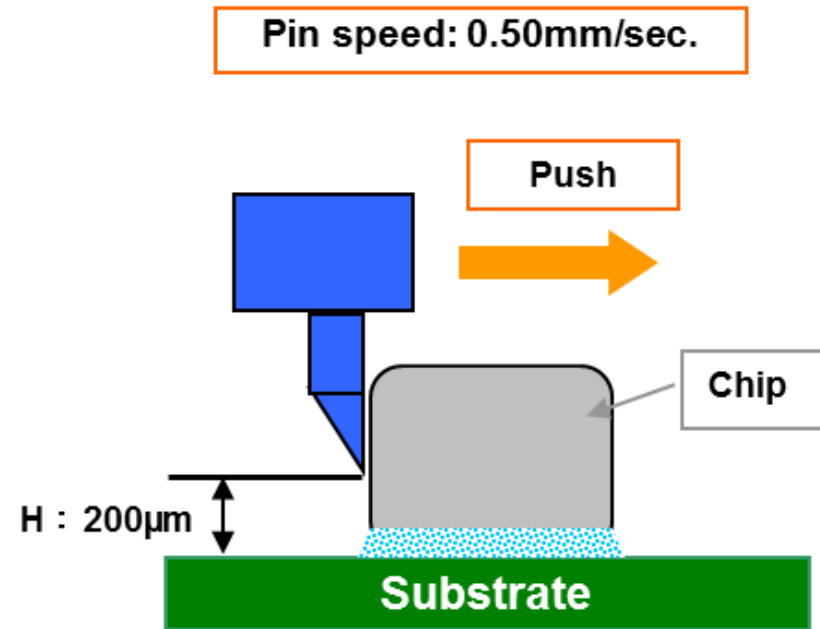
Schematic of shear test
