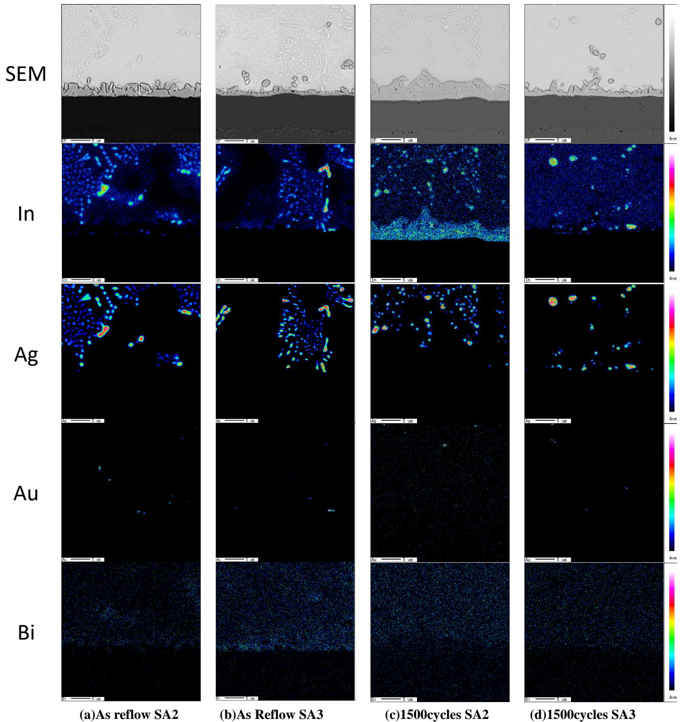
Figure 12- Solder Joint Interface of ENIG Board Finish: As Reflow and Thermal Cycled (In, Ag, Au, Bi Analyzed)
