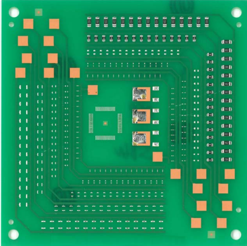
Test PCB for Thermal Cycling Test Evaluation(100x100mm)
