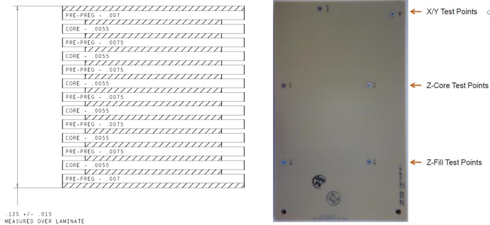
Figure 1: Test Vehicle Stack-up and Test Points on Test Vehicle
