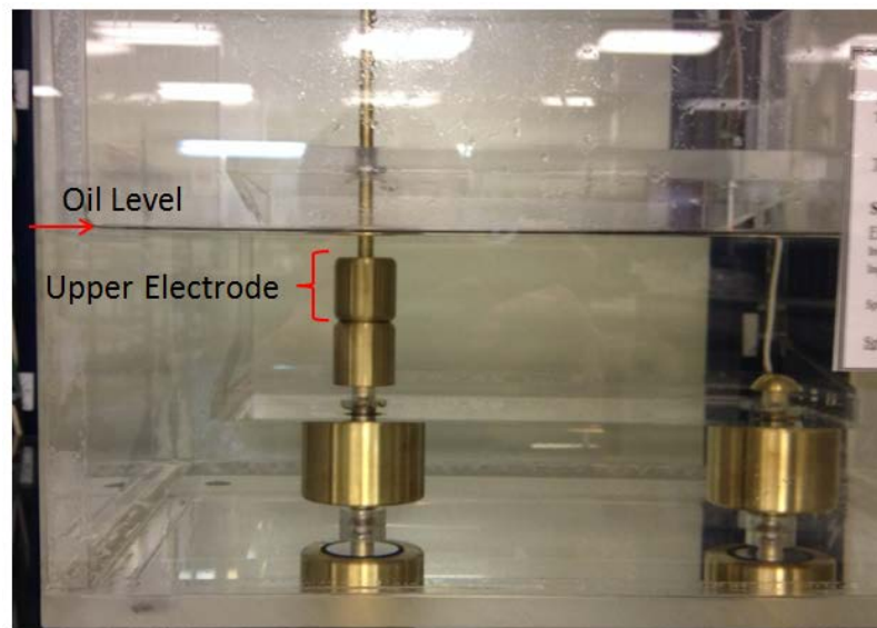
Oil bath and fixture sed for Controls
