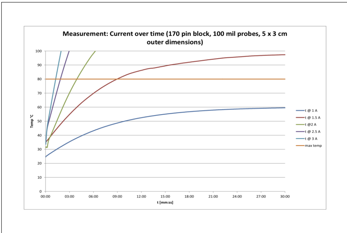
Figure 4 - Measured heat over time for a 170 pin config. transfer block
