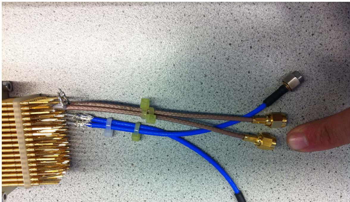
5mm length error (on purpose) to demonstrate the phase error in time domain
