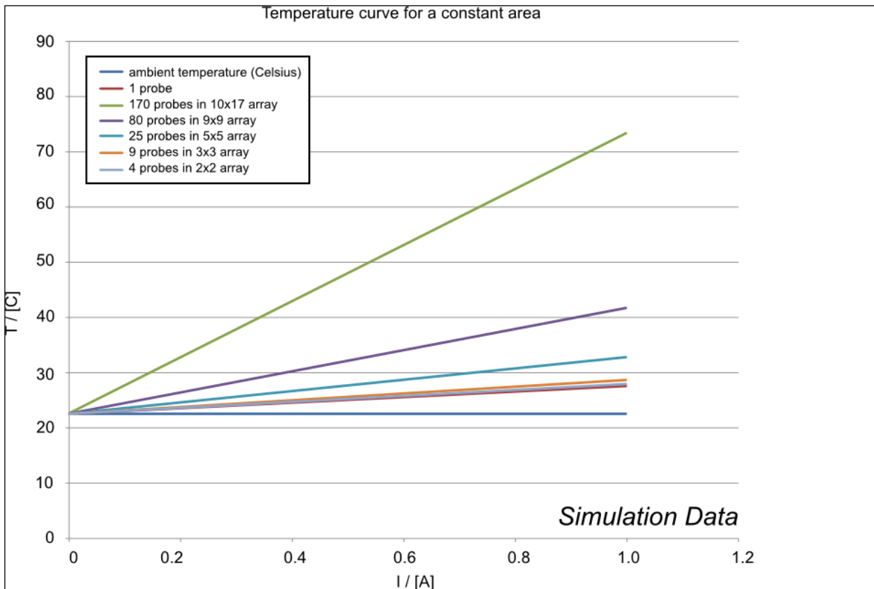
Figure 7 - Temperature (1 probe) for a constant area
