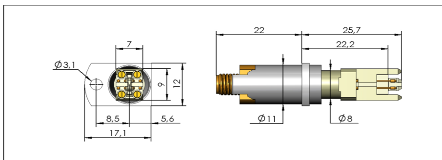
Figure 14 - High Speed Digital probe for a data connector
