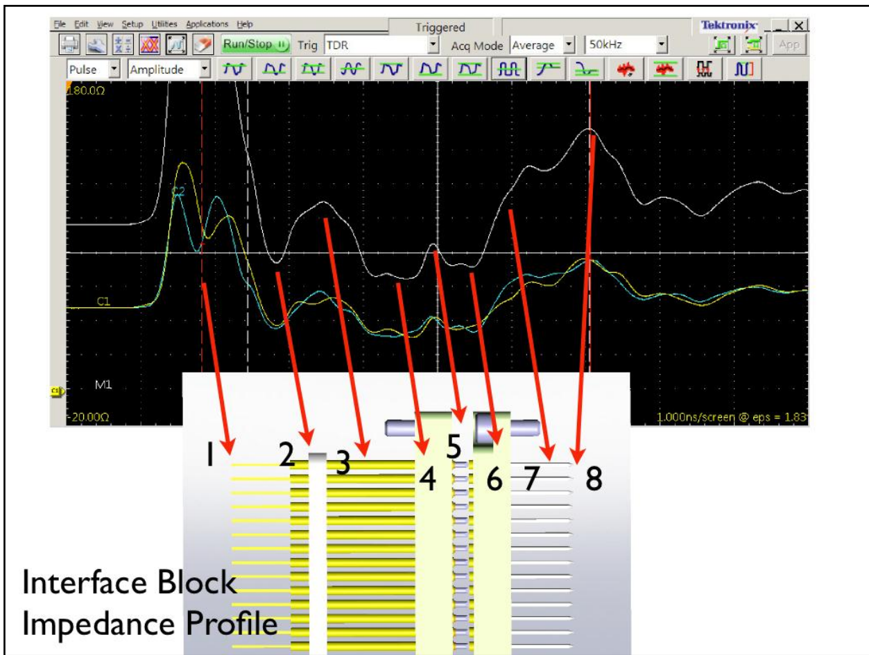
Figure 13 - Impedance profile for a 170 pin interface block
