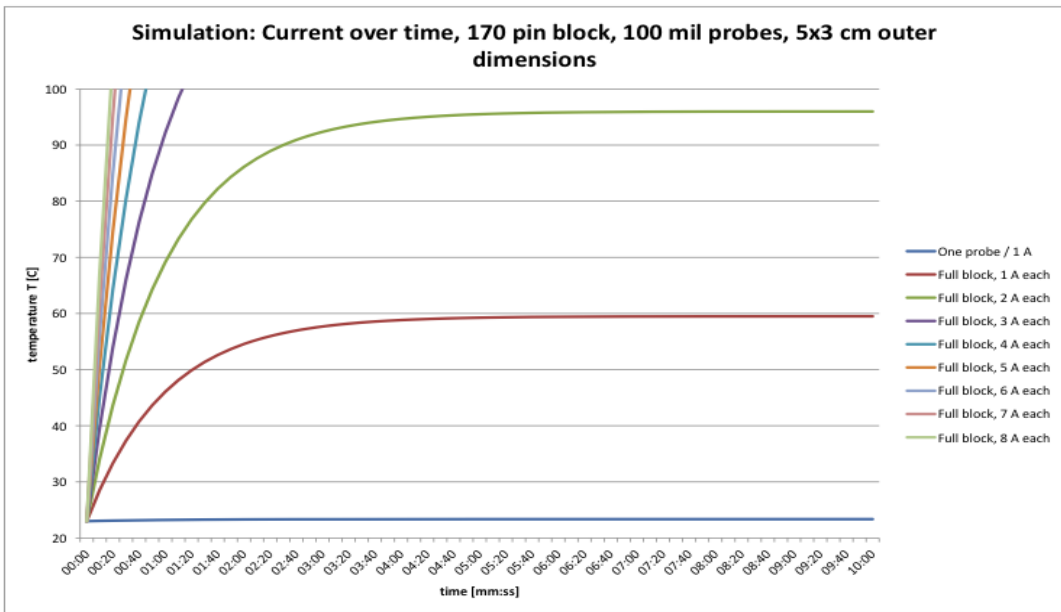
Figure 3 - Simulated heat over time for a 170 pin config. transfer block
