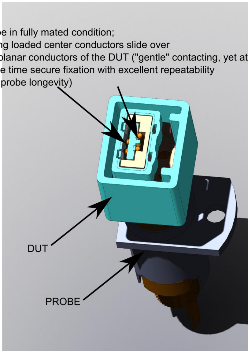
Figure 15 - Probe in fully-mated condition
