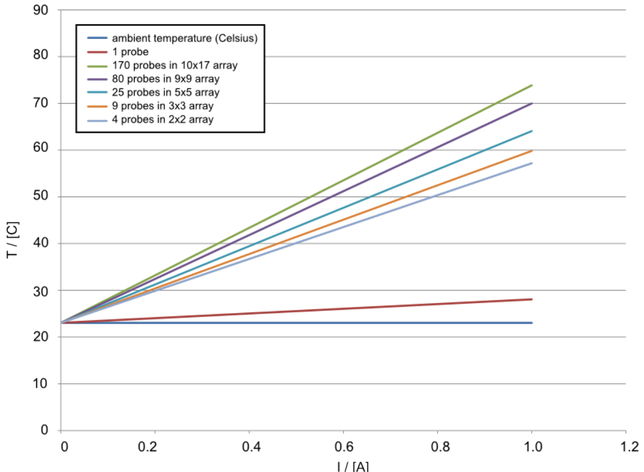
Temperature curve for constant pitch
