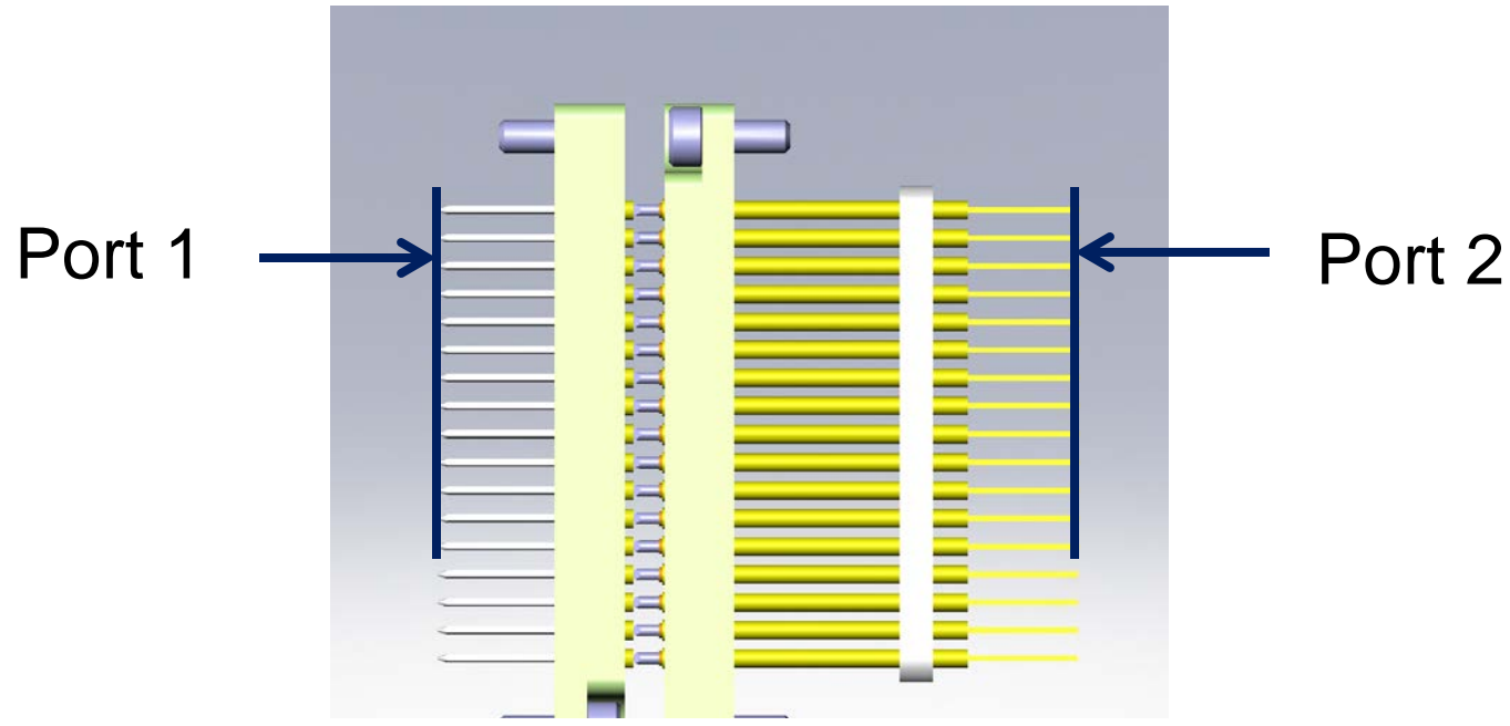
Cutplane view of the 170 pin block (in CST Microwave Studio) To show the references planes which are used for the simulation and the measurement
