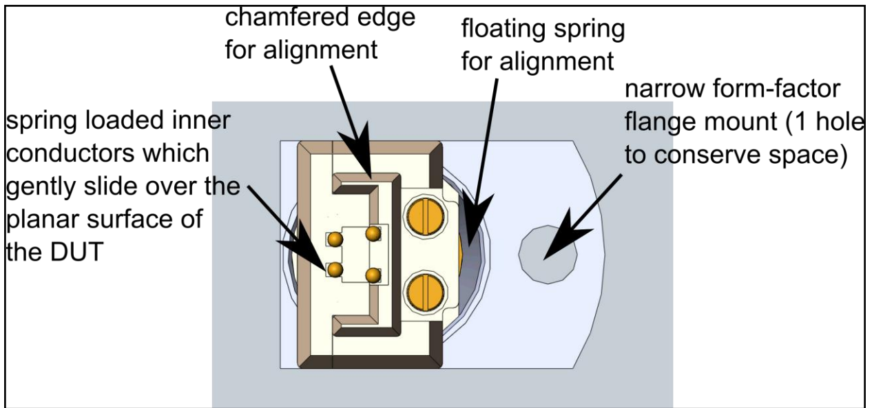
Figure 16 - Probe alignment features
