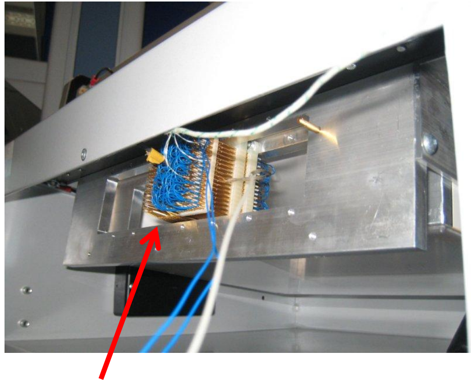
170 pin interface block with thermocouple element in a real life test Fixture (no test lab mockup)
