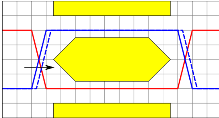
Figure 10 - Eye pattern degradation due to phase error / skew in the inverted signal
