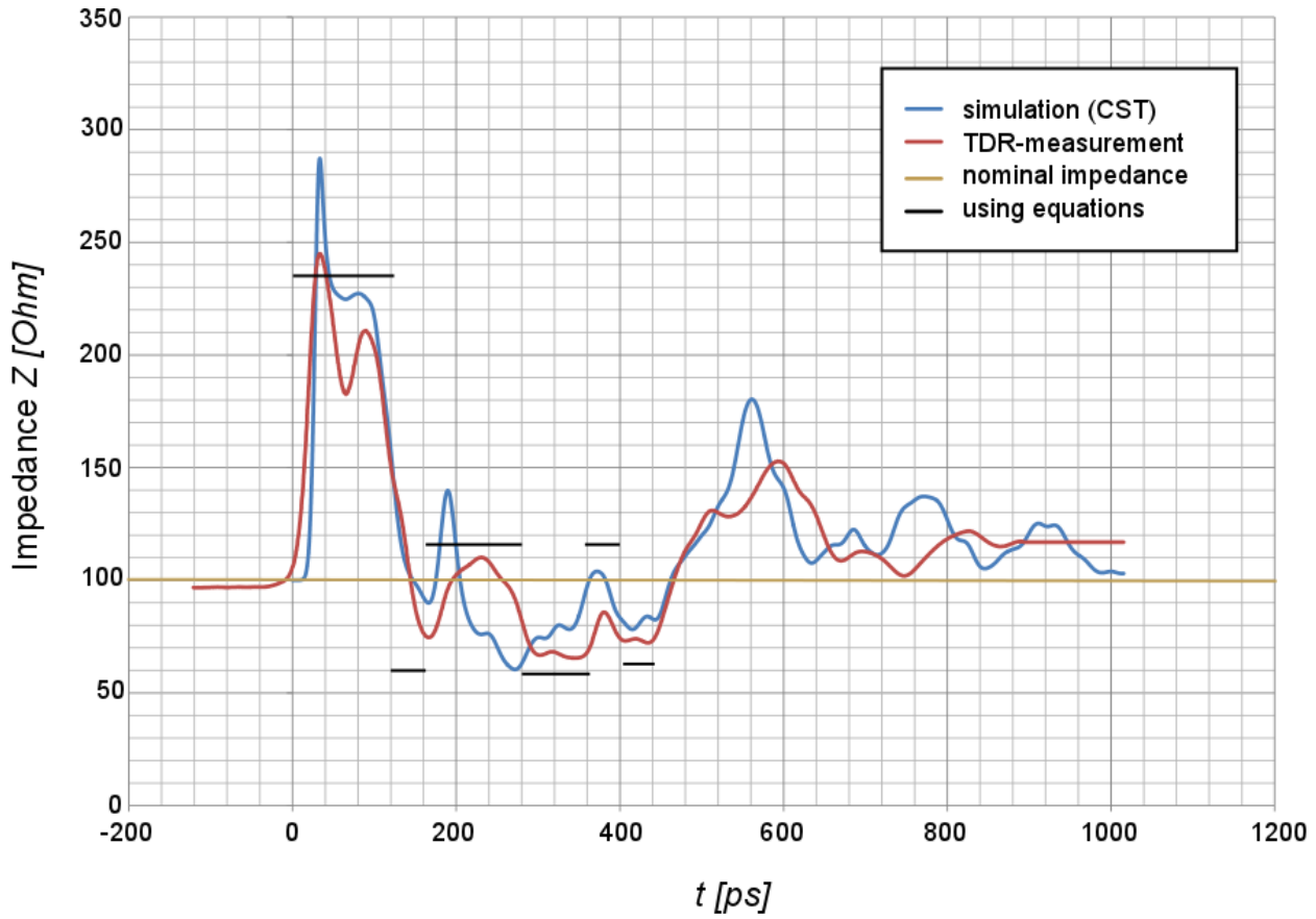
Figure 12 - Simulation vs. measurement comparison
