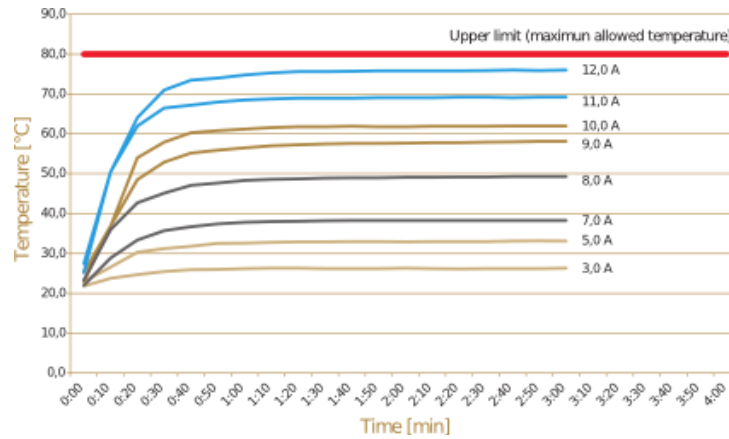
Figure 9 - Time / heat diagram (sample diagram) for various currents [ING10]
