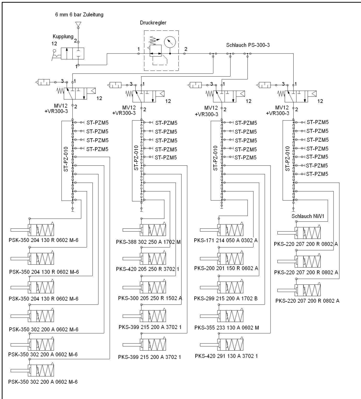
Figure 19 - Schematic for contacting 19 pneumatic probes in 4 groups
