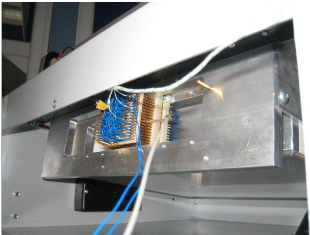
Figure 6 - Interface blocks installed in a regular mechanical test fixture with attached thermocouple sensor
