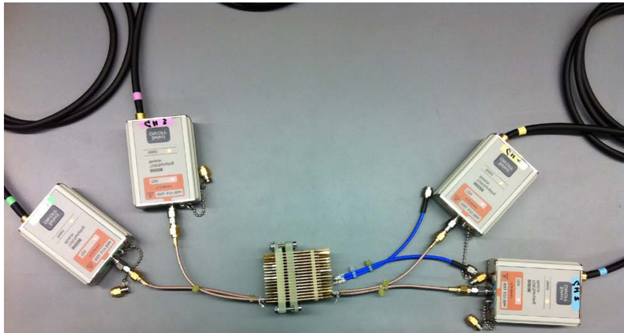
Figure shows the TDR detector heads (30 GHz) and the DUT (pylon block with 170 probes)
