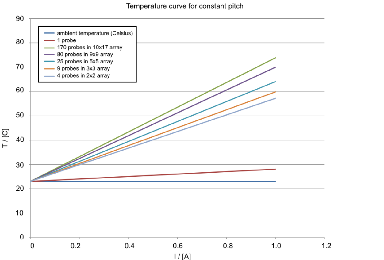
Figure 8 - Temperature (1 probe) for a constant pitch
