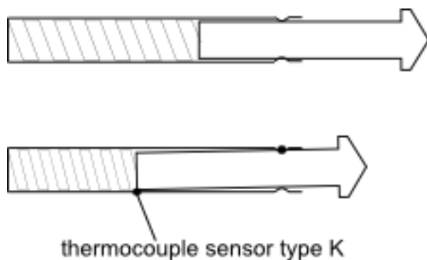
Figure 5 - Measurement point for the thermocoupler
