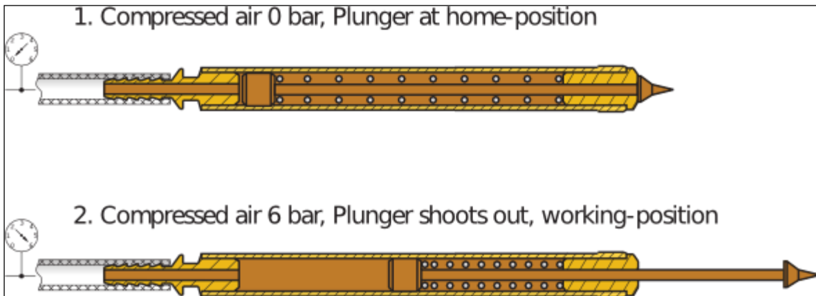
Figure 17 - Working principle of a pneumatic test probe [ING10]
