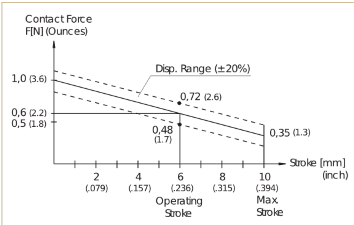
Figure 18 - Spring-force diagram (sample) for a pneumatic probe [ING10]
