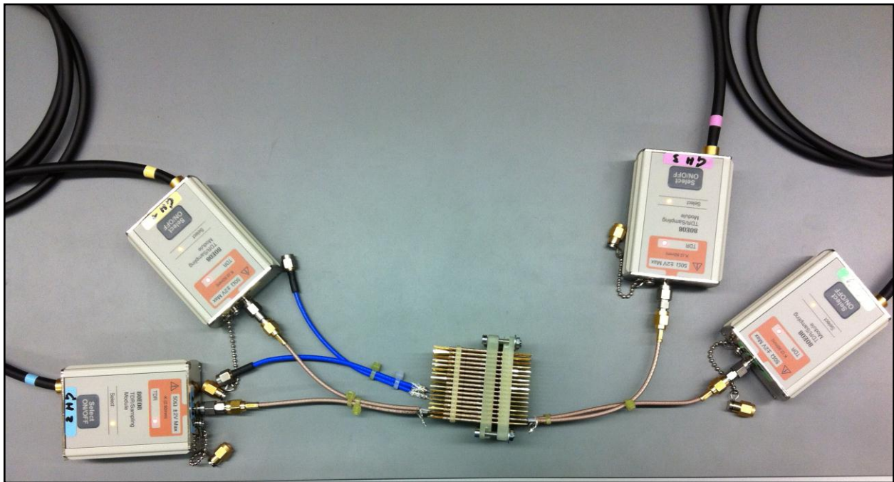
Figure 11 - Measurement setup with 4 x 30 GHz detector heads
