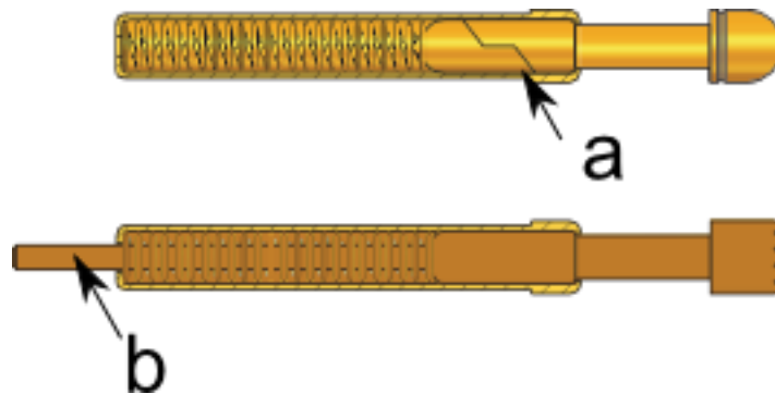
Figure 2 - Basic principles to lower the resistance of a high current probe [ING10]
