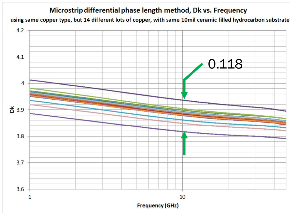
Circuits using rough copper; RMS = 2.8 microns
