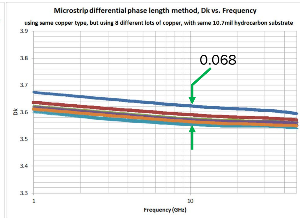
Circuits using smooth copper; RMS = 0.9 microns
