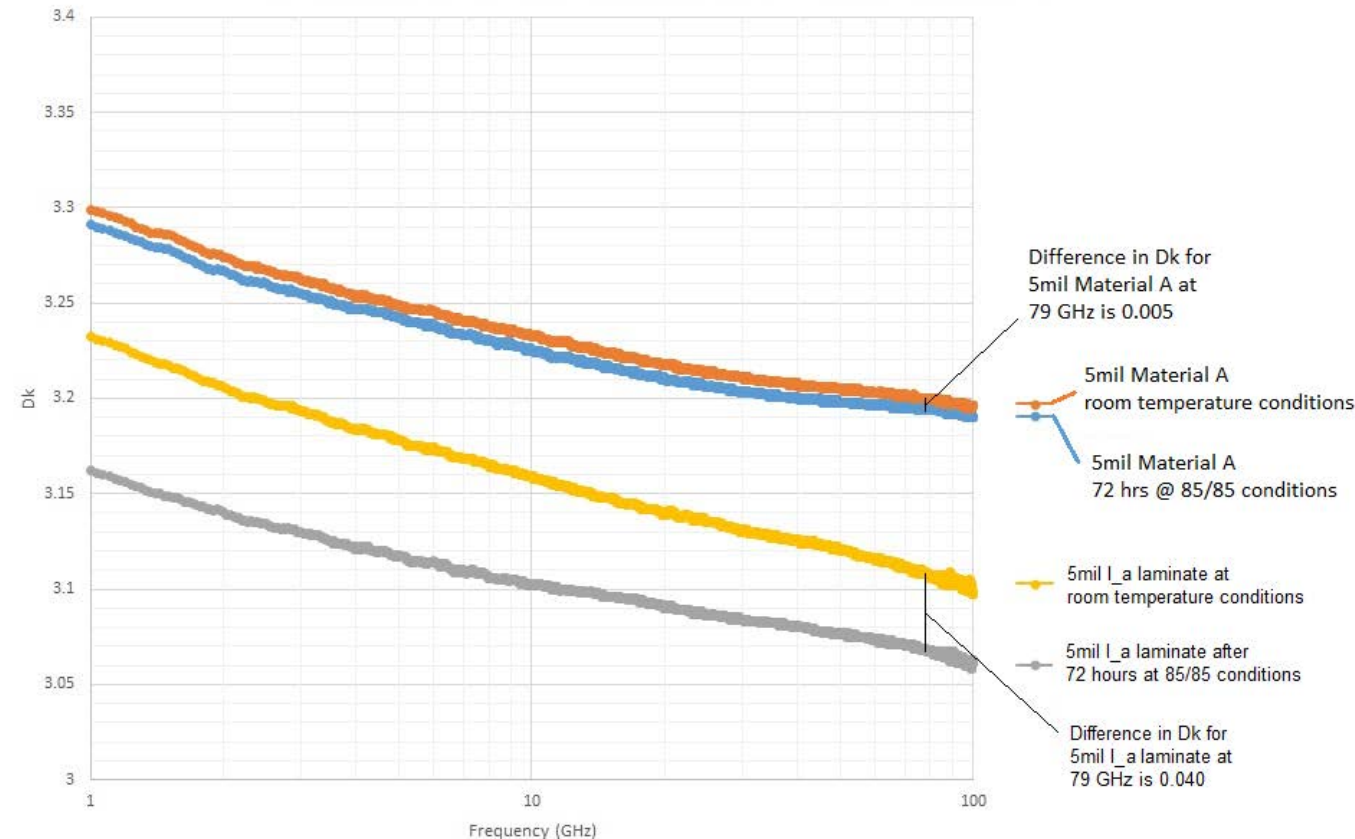
Microstrip differential phase length method, Dk vs. Frequency Circuits conditioned at room temperature and 24 hours @ 85C / 85% RH
