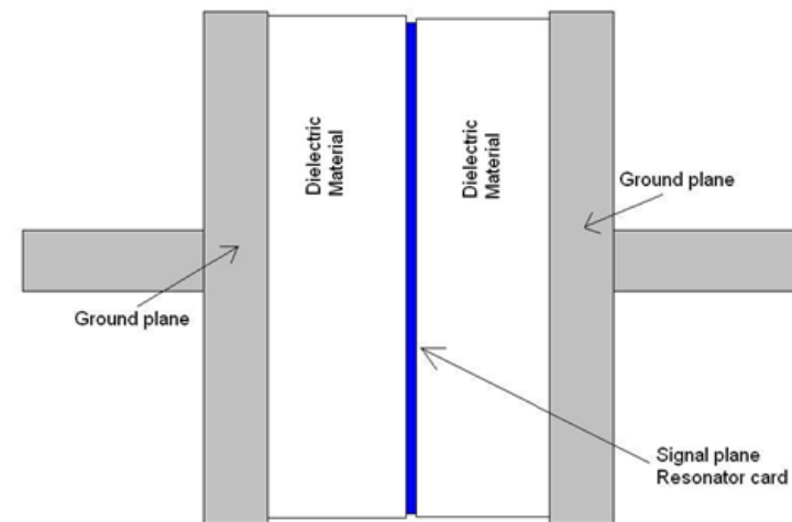
Side view of resonator card clamped into test fixture
