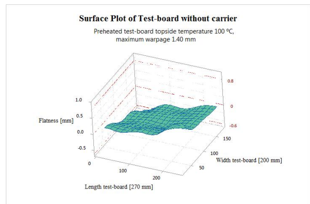
Figure 16: The test-board warpage when it is not placed into a carrier.
