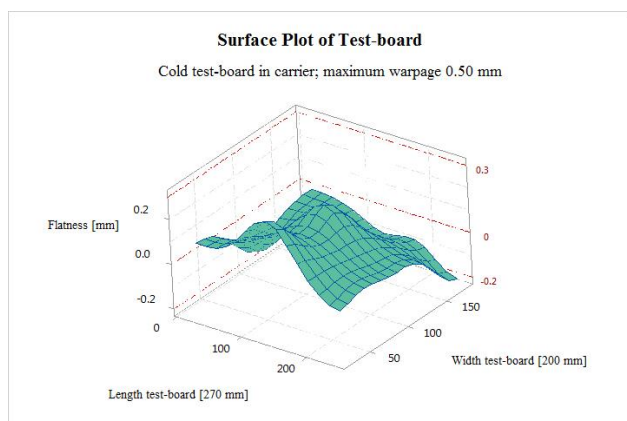
Figure 14: The warpage of a cold test-board after two times reflow.
