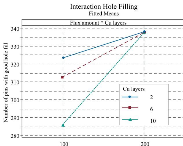
Figure 3: The flux amount is critical for the hole filling.
