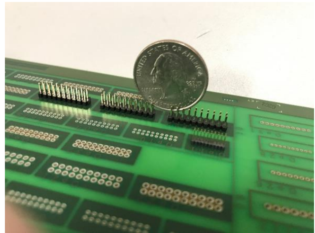
Figure 1: Test-board.
