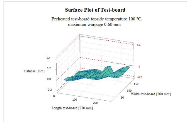
Figure 15: The test-board, although preheated (100 °C), remains relatively flat due to the carrier.
