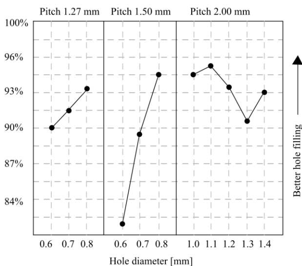
Figure 4: Hole filling for different barrel diameters (higher score is better).
