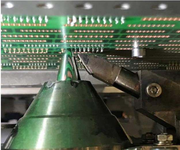
Figure 5: A wettable nozzle with SDC unit.
