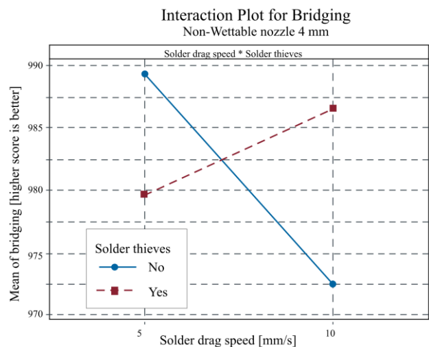
Figure 7: At high drag speeds (10 mm/s) solder thieves have a benefit (a higher score is less bridging is better)
