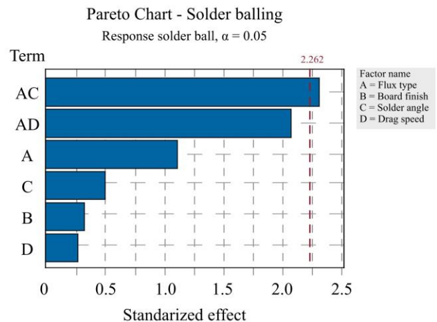
Figure 10: Pareto chart for solder balling. There are interactions due to the different flux properties.
