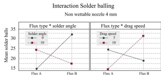
Figure 11: The average number of solder balls – the lower the score the better.
