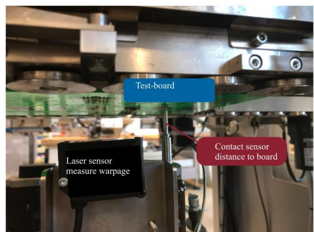
Figure 17: test setup with laser and contact sensor.
