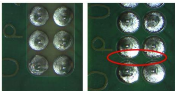
Figure 9: Left the solder mask removed, right with solder mask and solder ball.
