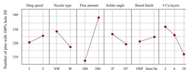
Figure 2: shows the impact on hole-fill for different parameters – the higher score the better hole filling.
