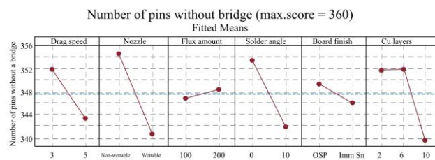
Figure 6: Impact of the different parameters on bridging.
