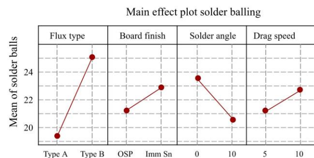
Figure 12: Overall analysis of solder balling showing that the flux type has a major impact.
