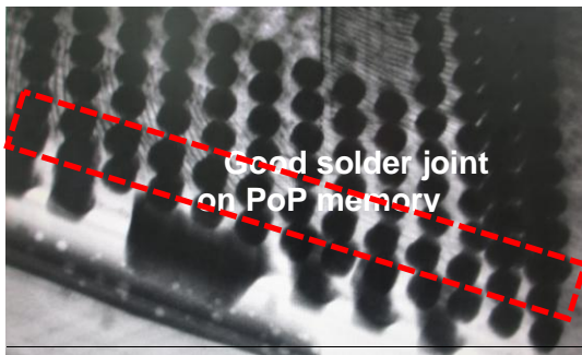
(a) X-ray image of POP using SMT 256
