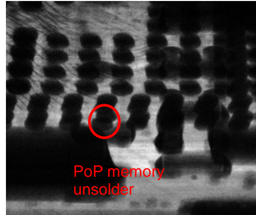
Figure 4. X-ray Image of Assembled POP Using Solder Paste and Flux.
