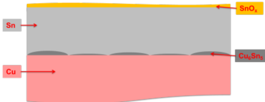
Illustrated presentation of an as received pad
