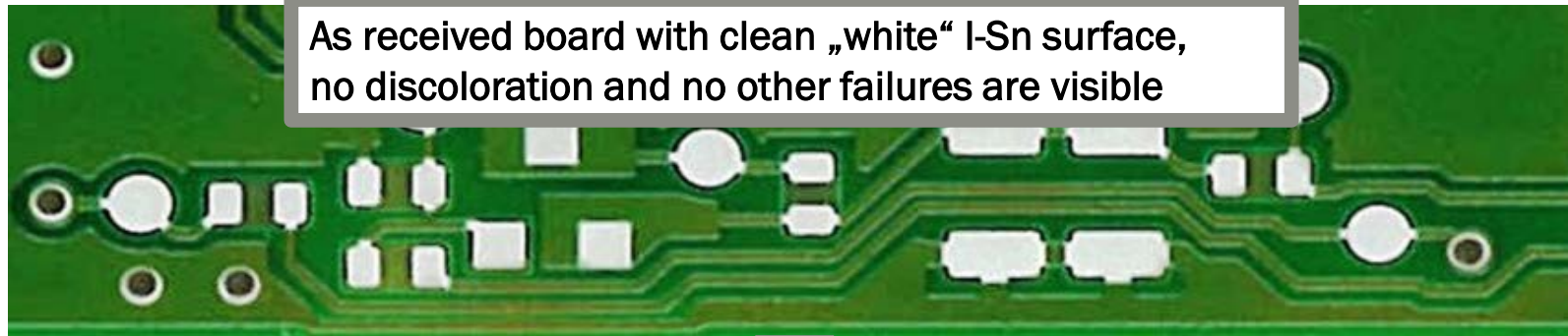
Illustrated presentation of an as received pad
