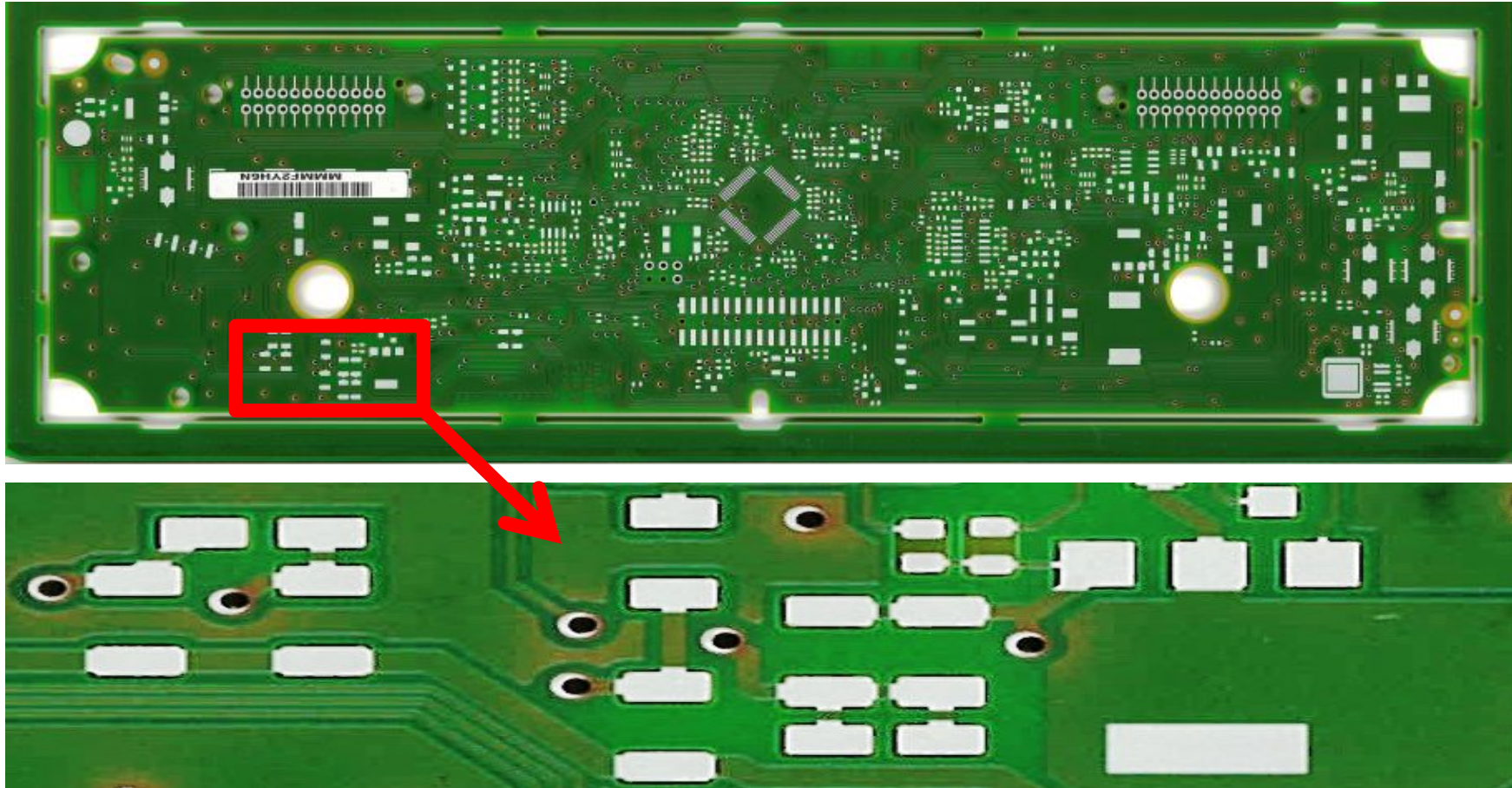
After 1 st reflow the non-soldered look clean „white“, no discoloration and no other failures are visible
