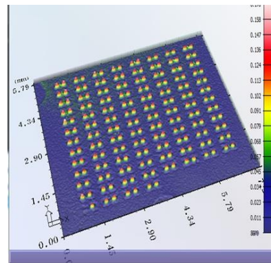
Figure 8: Overview of paste deposits 008004'' (0201mm)
