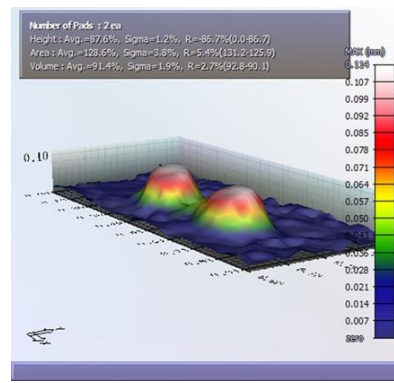
Figures 9: Individual Paste Deposits 008004'' (0201mm)
