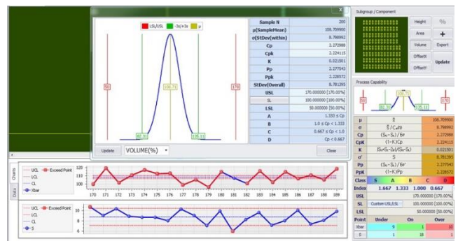
Figure 6: Volume Results 90-Degrees 008004'' (0201mm)
