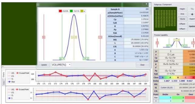
Figure 4: Volume Results 0-Degrees 008004'' (0201mm)
