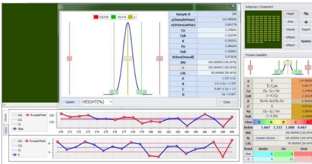
Figure 5: Height Results 0-Degrees 008004'' (0201mm)
