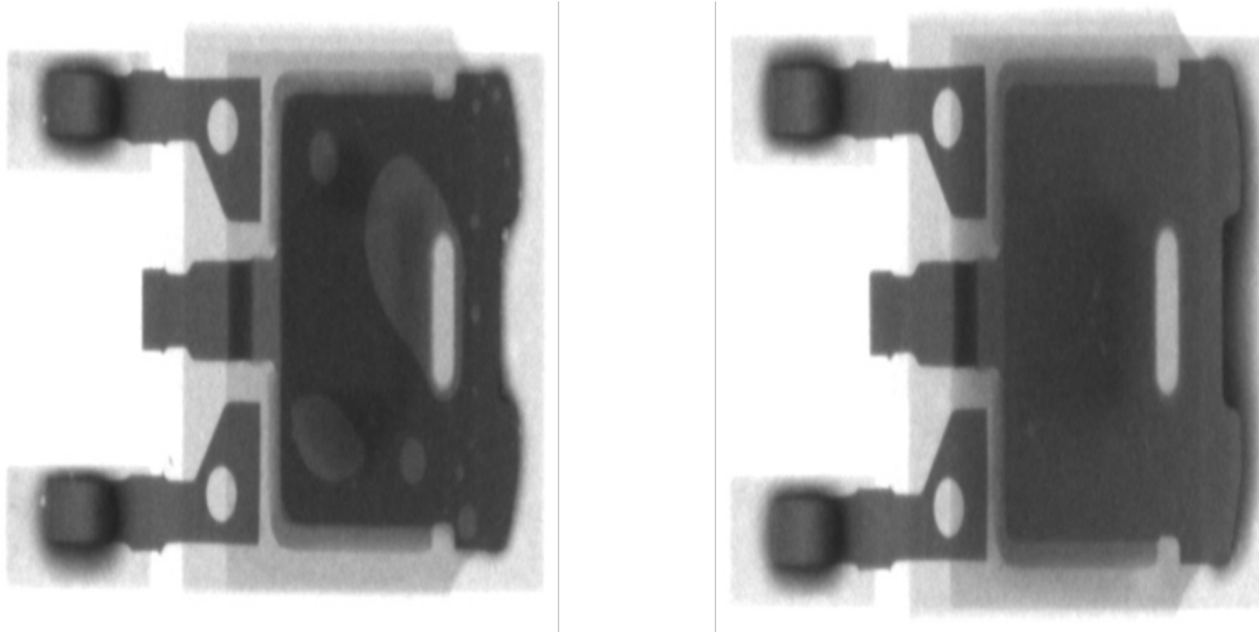
T0-252 Package with no vacuum (left) and 5 torr for 60 seconds vacuum (right)
